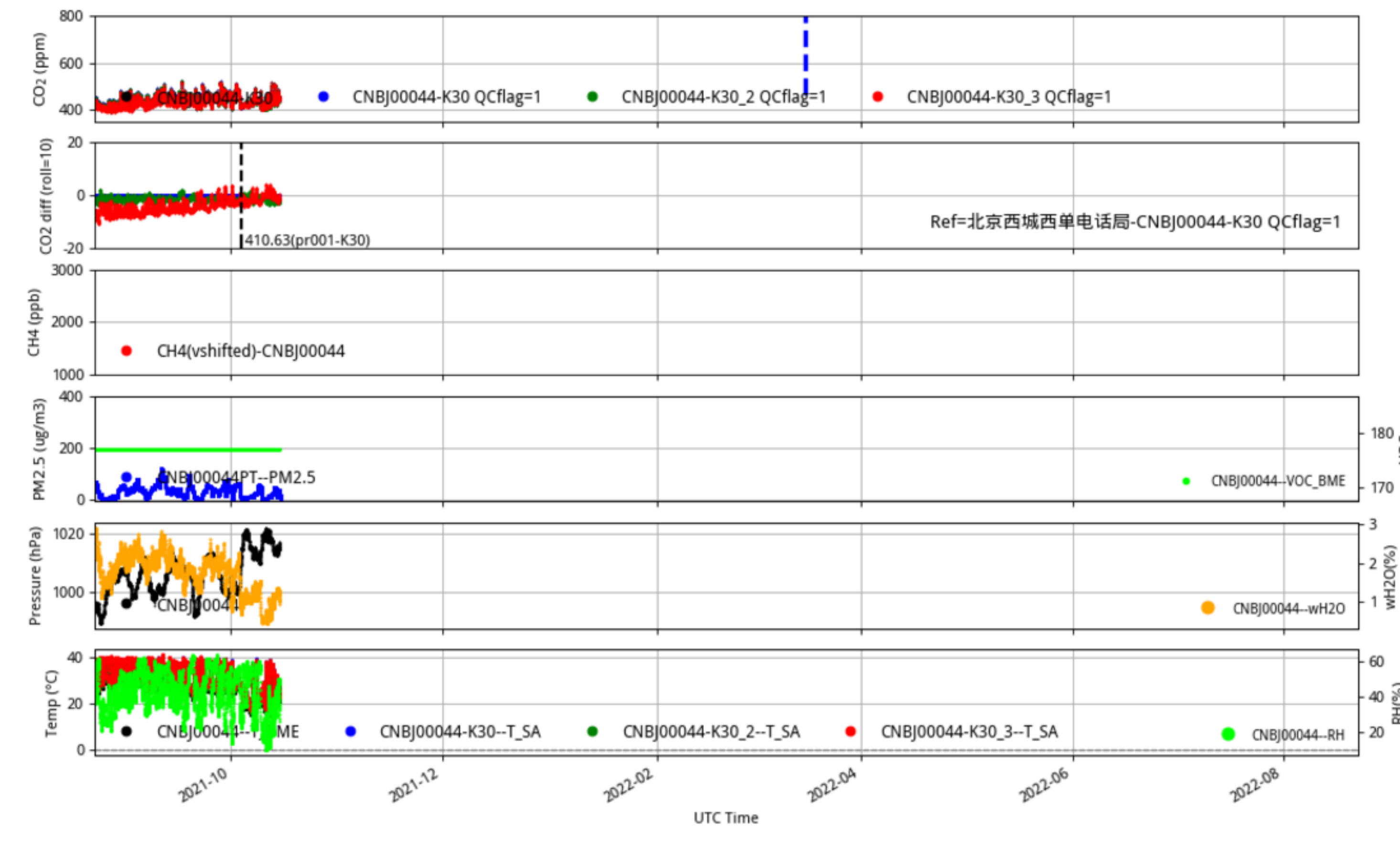
CNBj00044 JJJ_station tenmin/L2.1 CNBj00044--365-days
