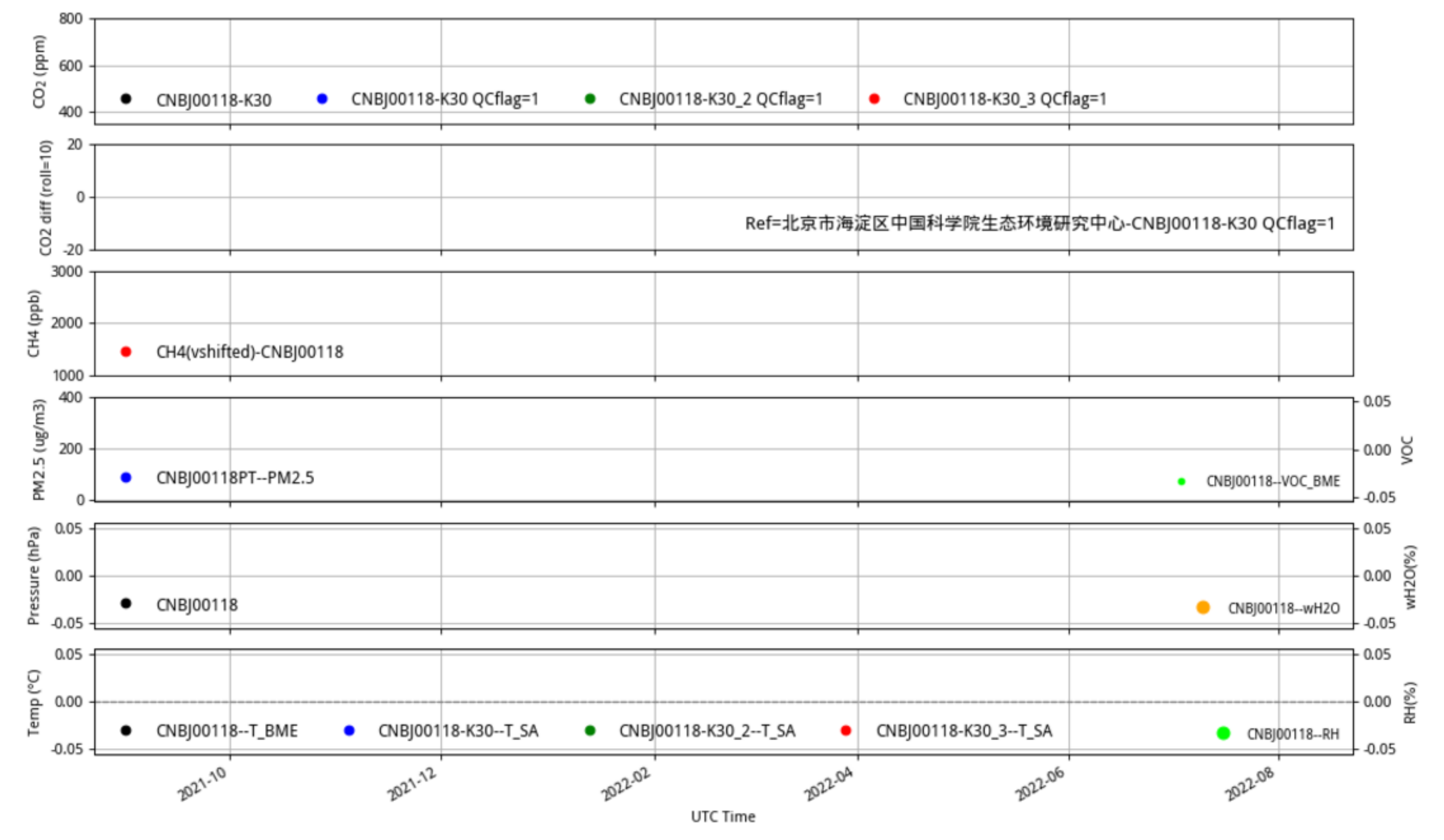
CNBj00118 JJJ_station tenmin/L2.1 CNBj00118--365-days
