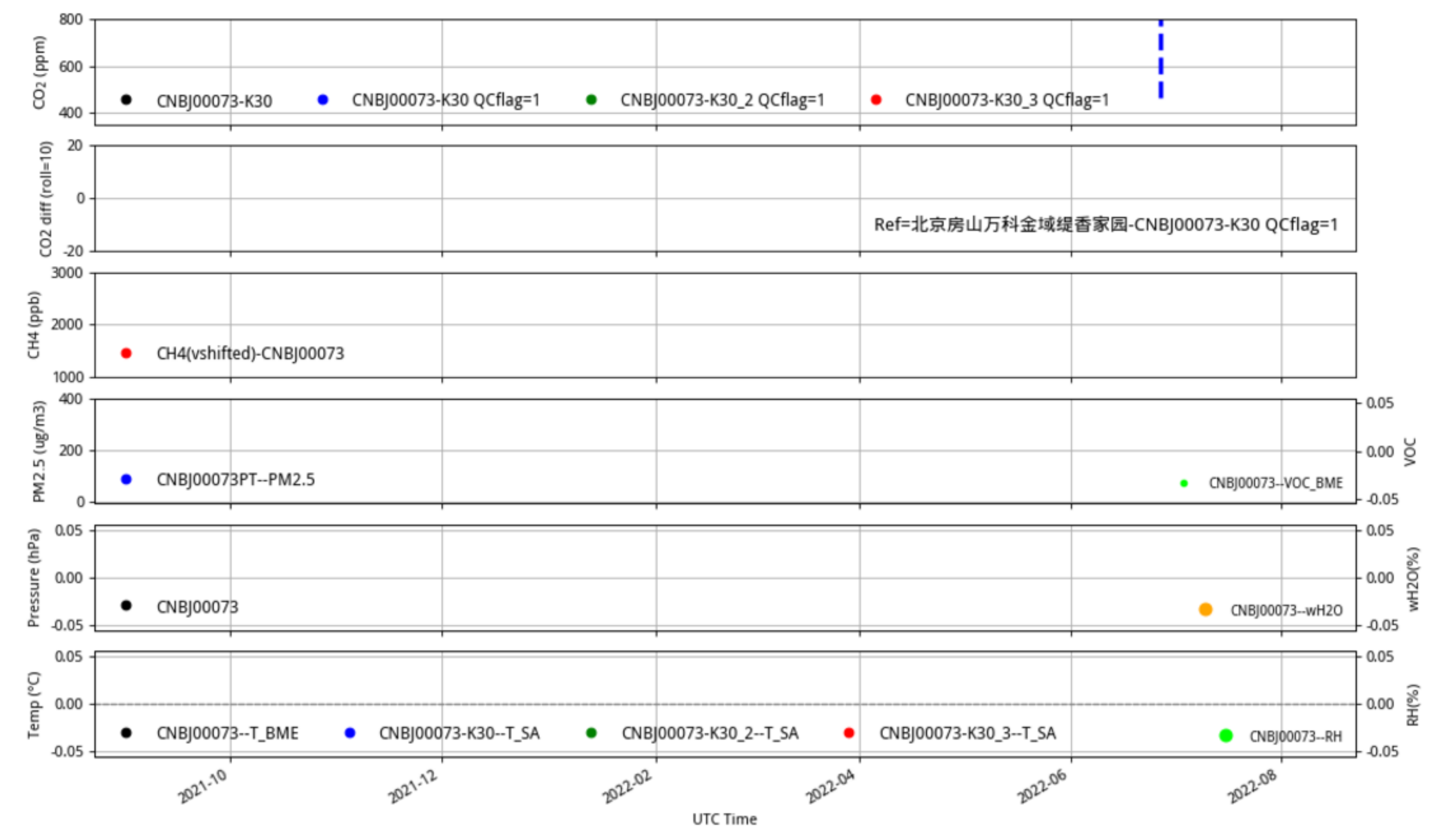
CNBj00073 JJJ_station tenmin/L2.1 CNBj00073--365-days
