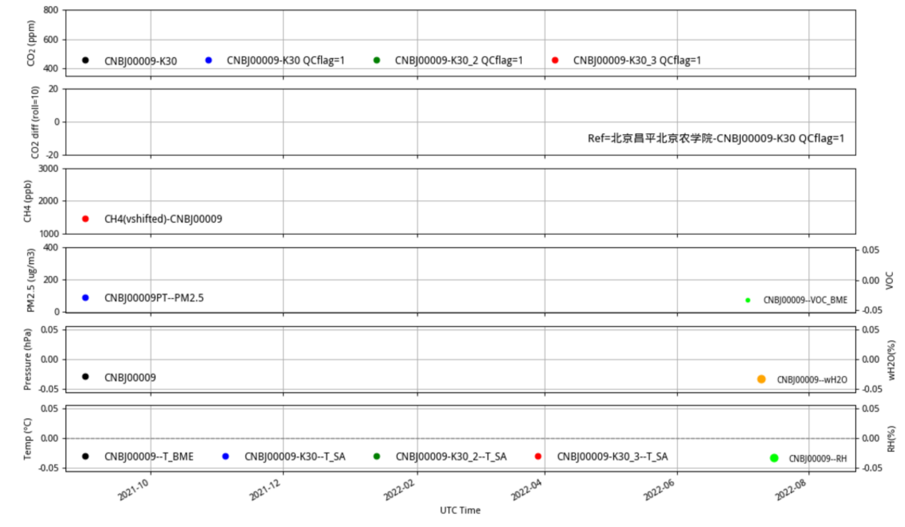
CNBj00009 JJJ_station tenmin/L2.1 CNBj00009--365-days
