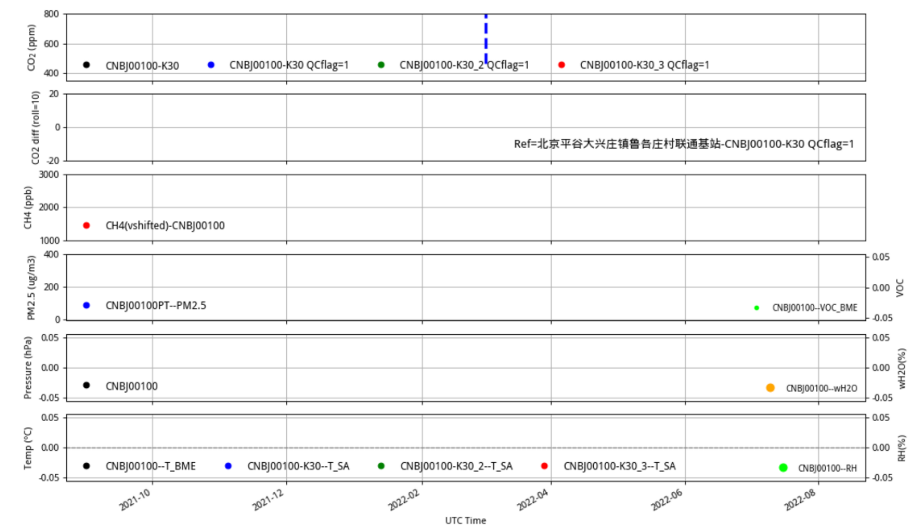
CNBj00100 JJJ_station tenmin/L2.1 CNBj00100--365-days
