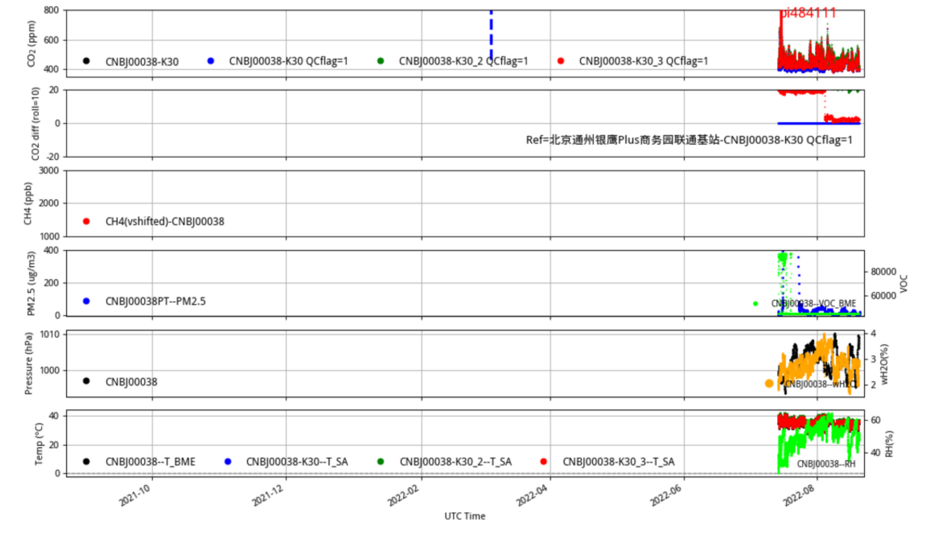
CNBj00038 JJJ_station tenmin/L2.1 CNBj00038--365-days
