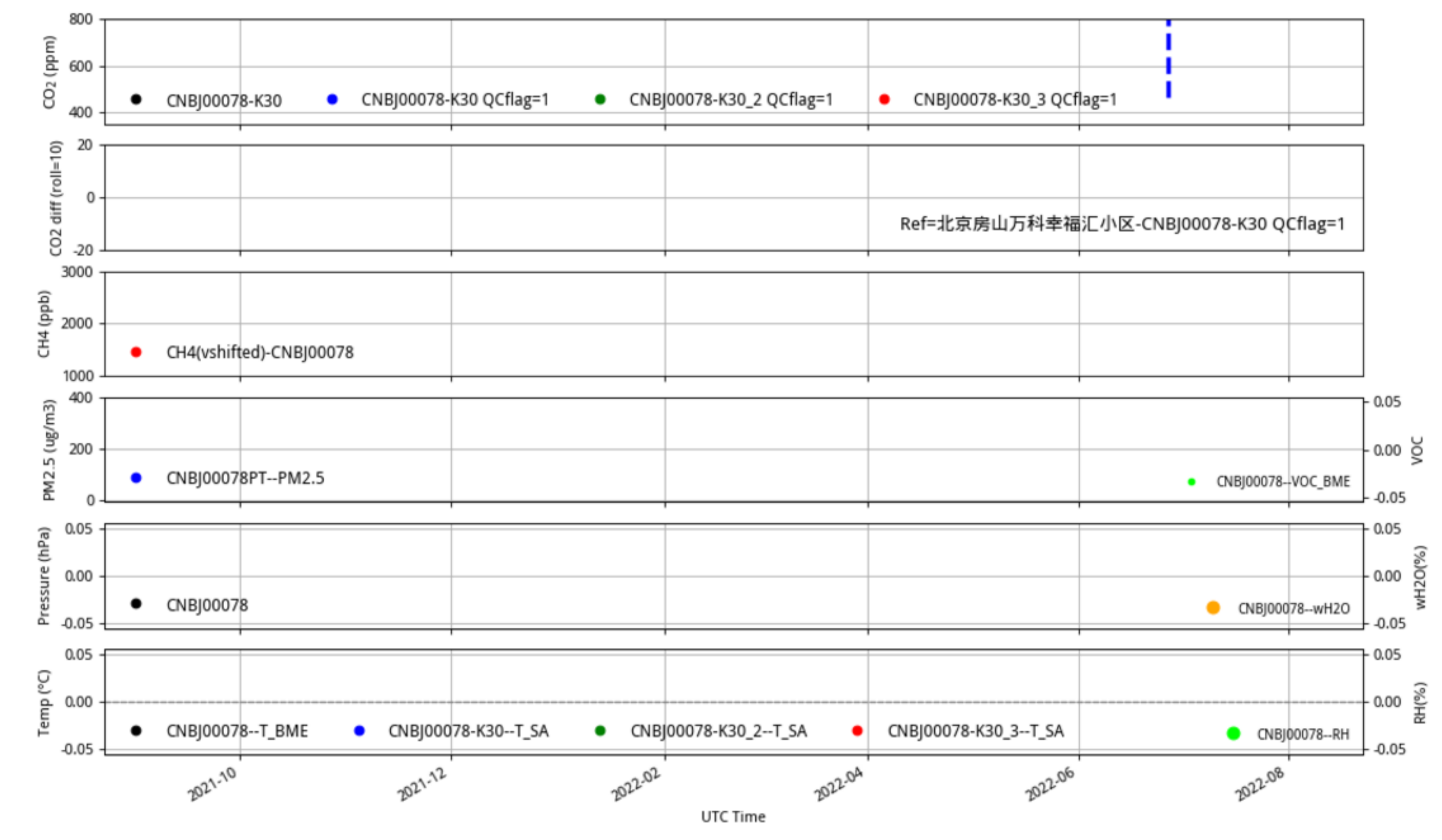
CNBj00078 JJJ_station tenmin/L2.1 CNBj00078--365-days
