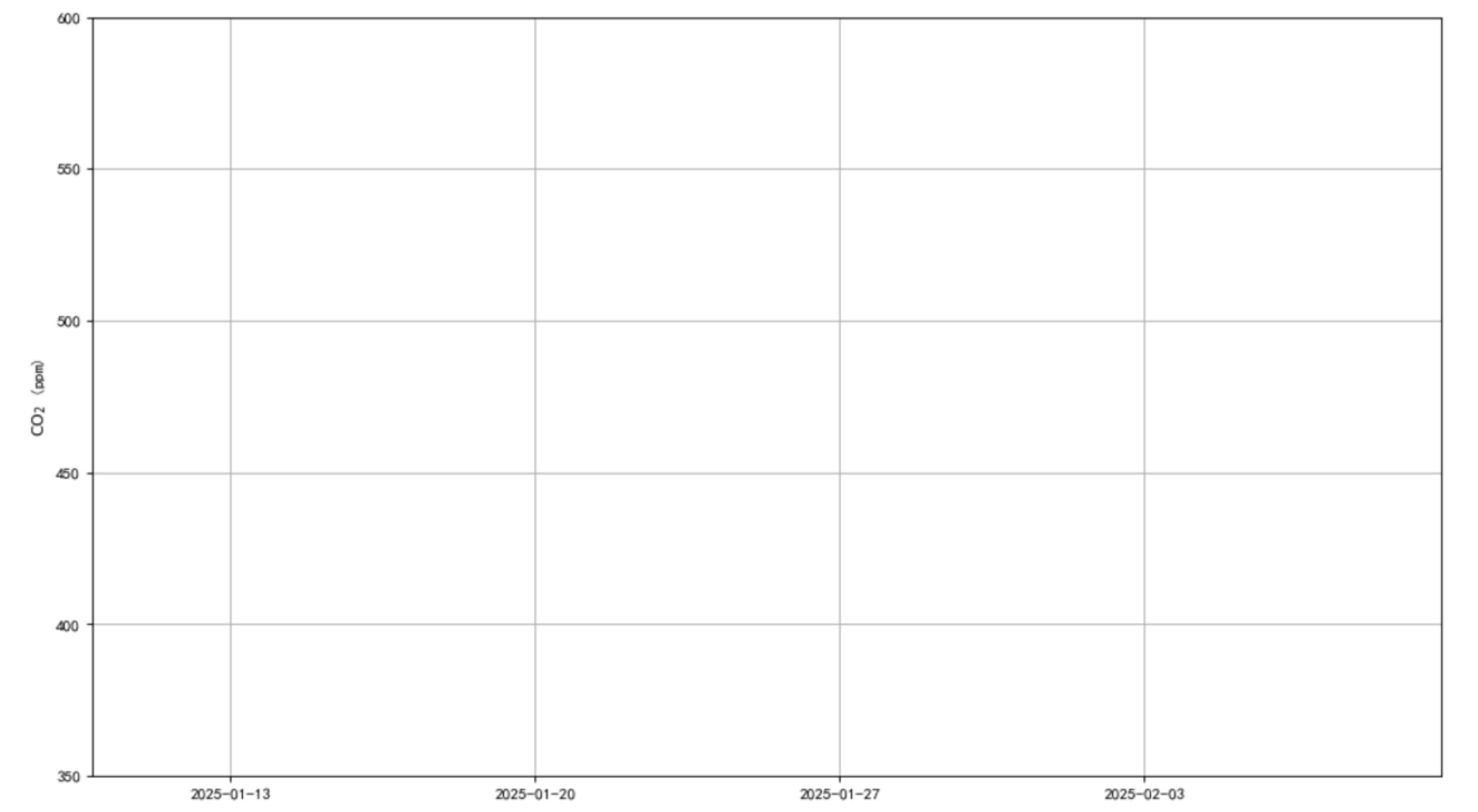
QH_Waliguan_CMAH2 hr/L2.0 for 1-month
