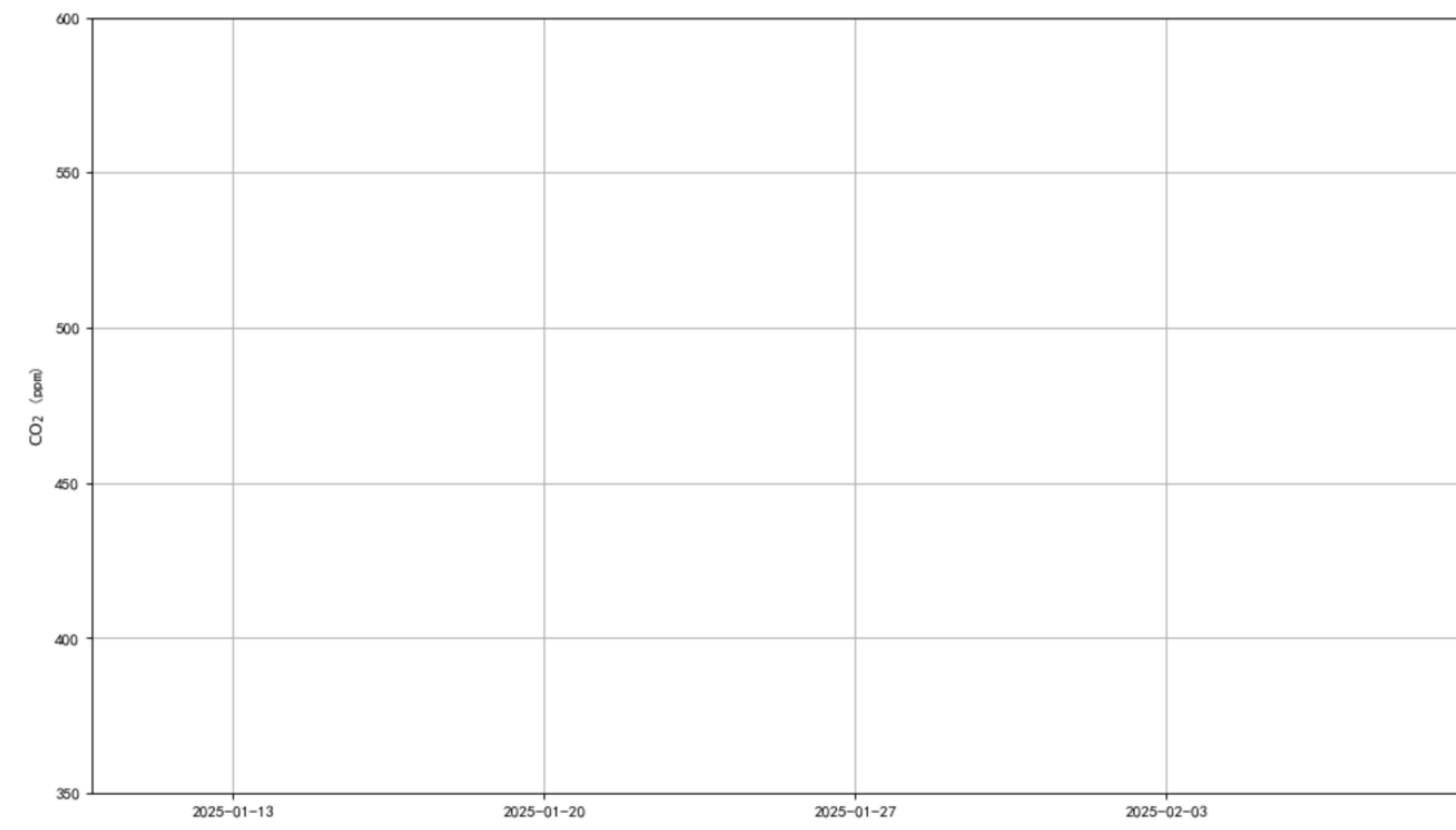
QH_Waliguan_CMAH1 hr/L2.0 for 1-month
