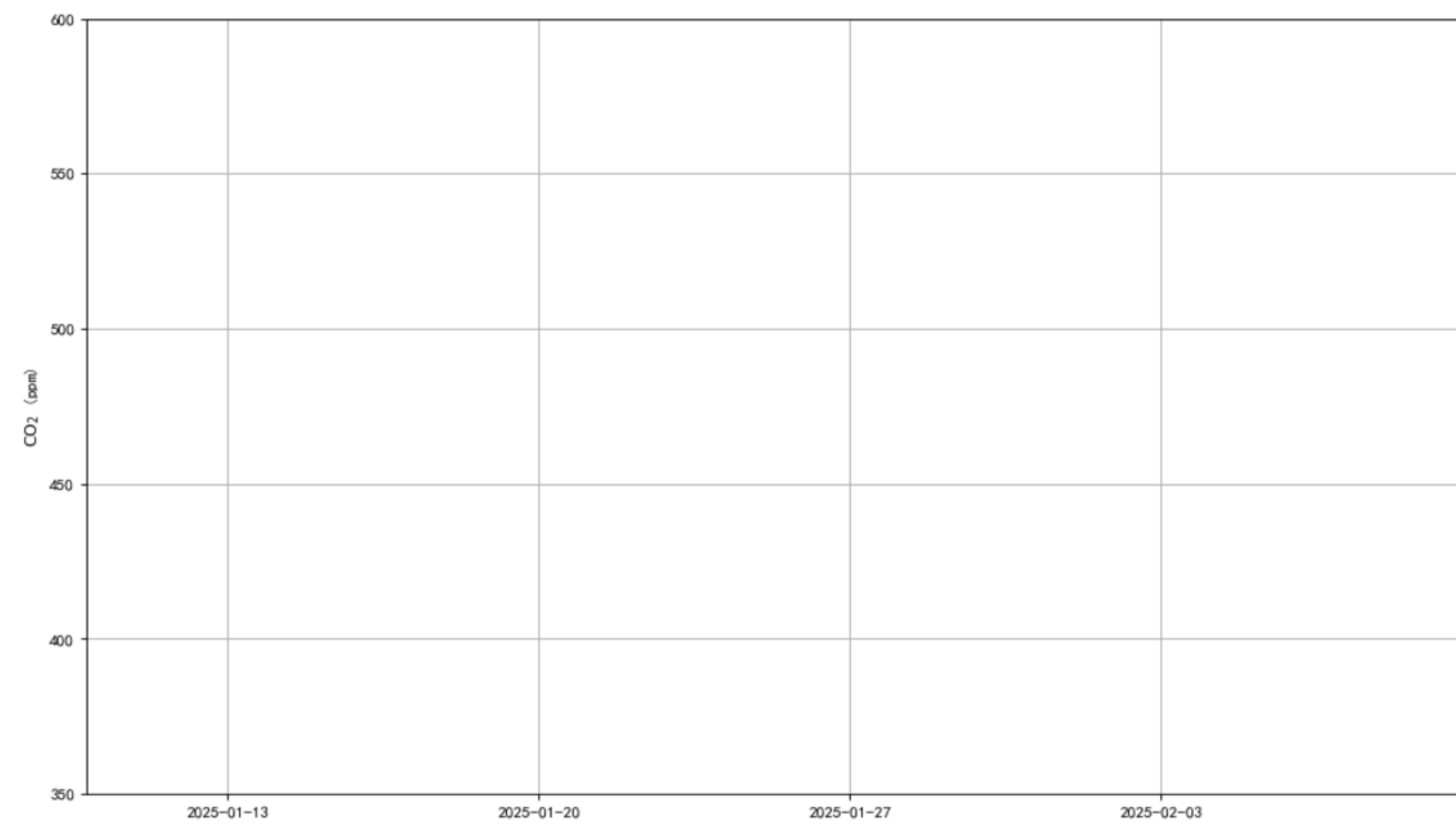
ZJ_LinAn_CMAH1 hr/L2.0 for 1-month
