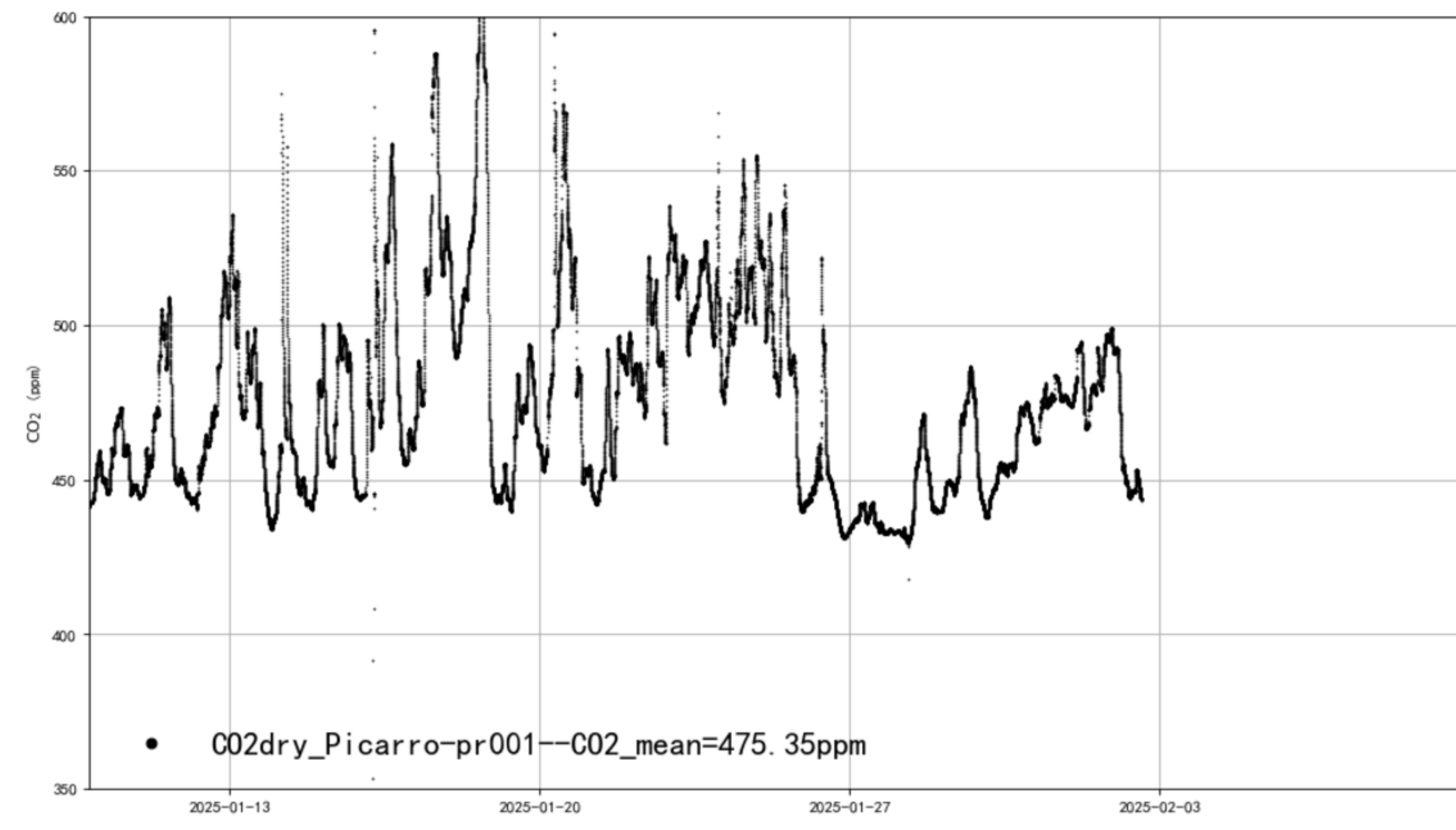
BJ_IAPLab617 min/L2.0 for 1-month
