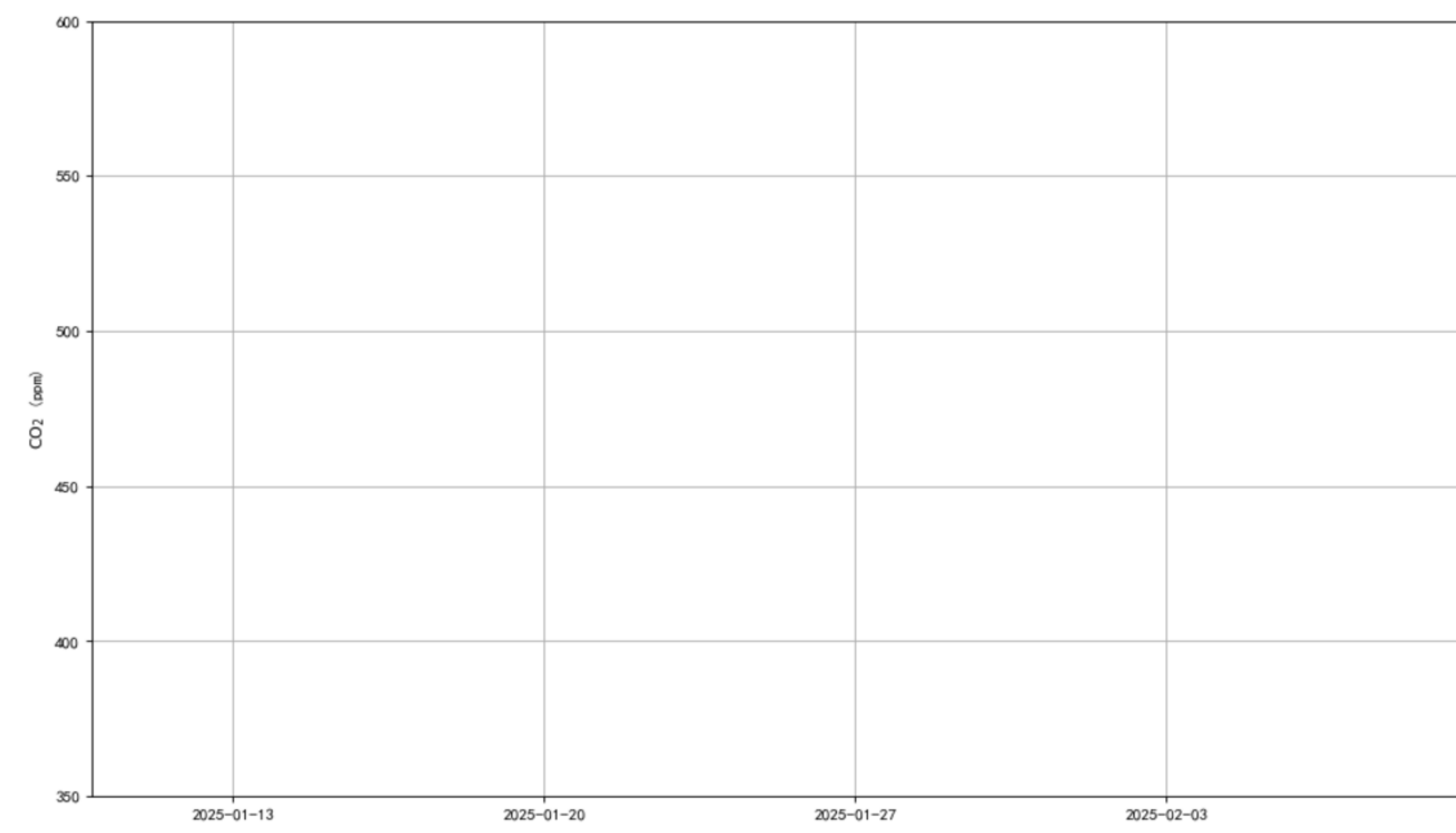
BJ_IAPTower_WINH2 min/L2.0 for 1-month
