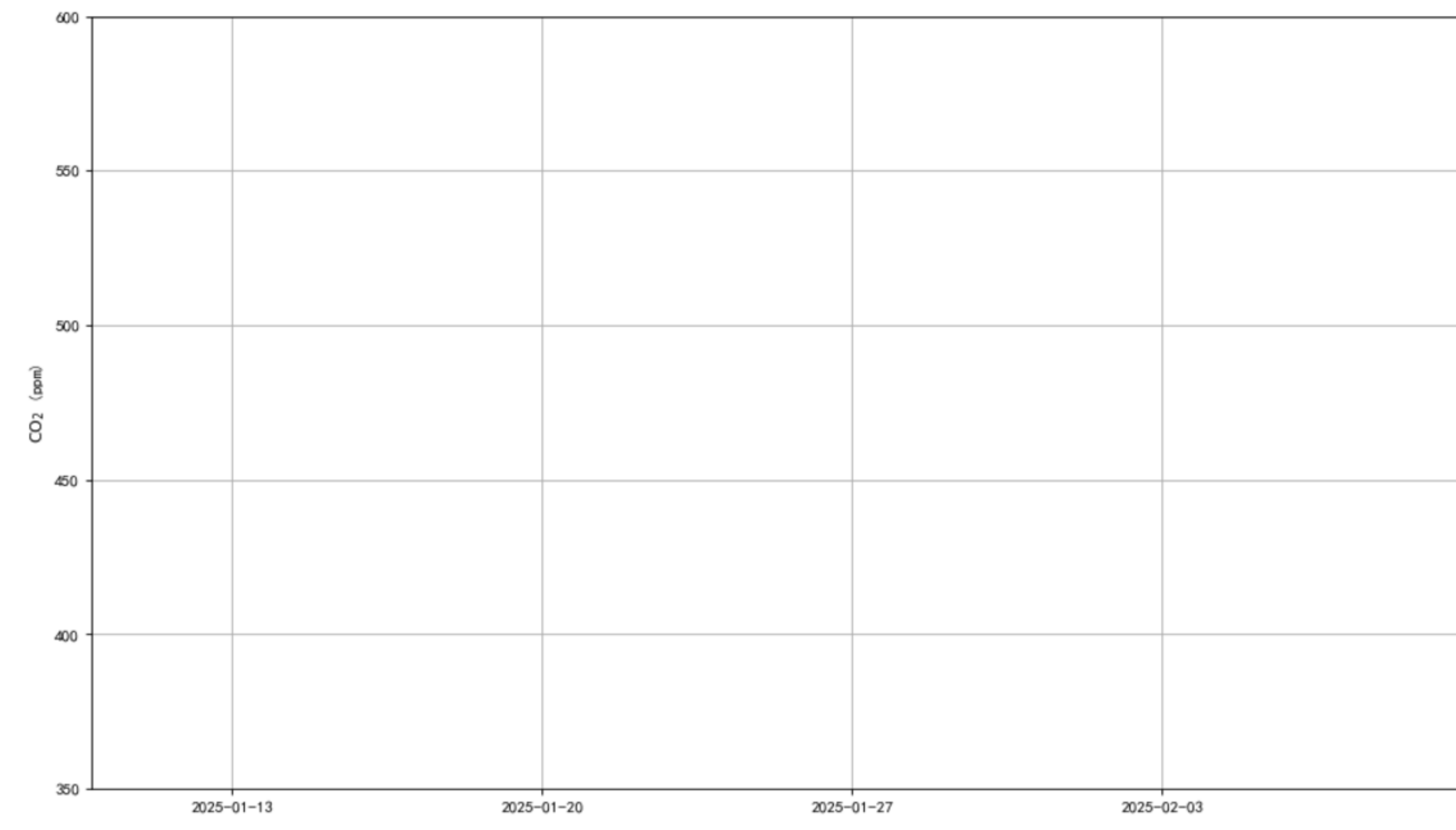
BJ_Shangdianzi_CMAH1 min/L2.0 for 1-month
