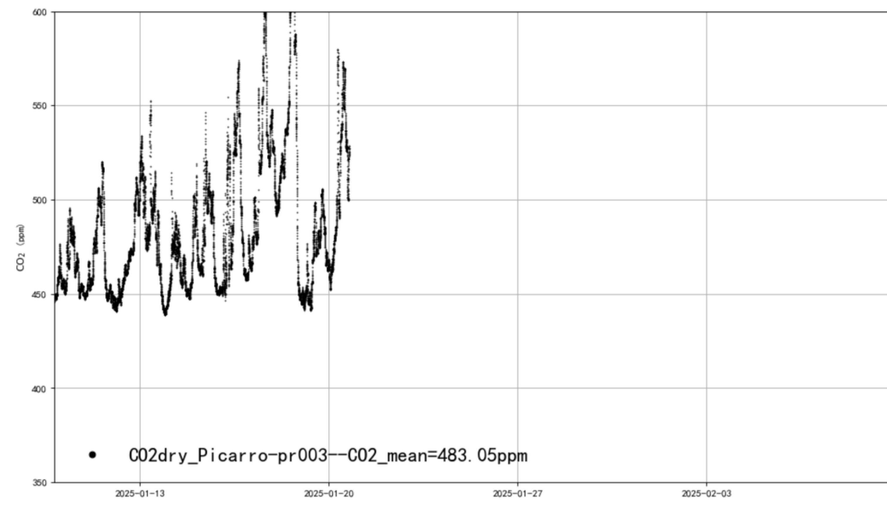
CNBJ_IAPTower_Picarro_collector min/L2.0 for 1-month
