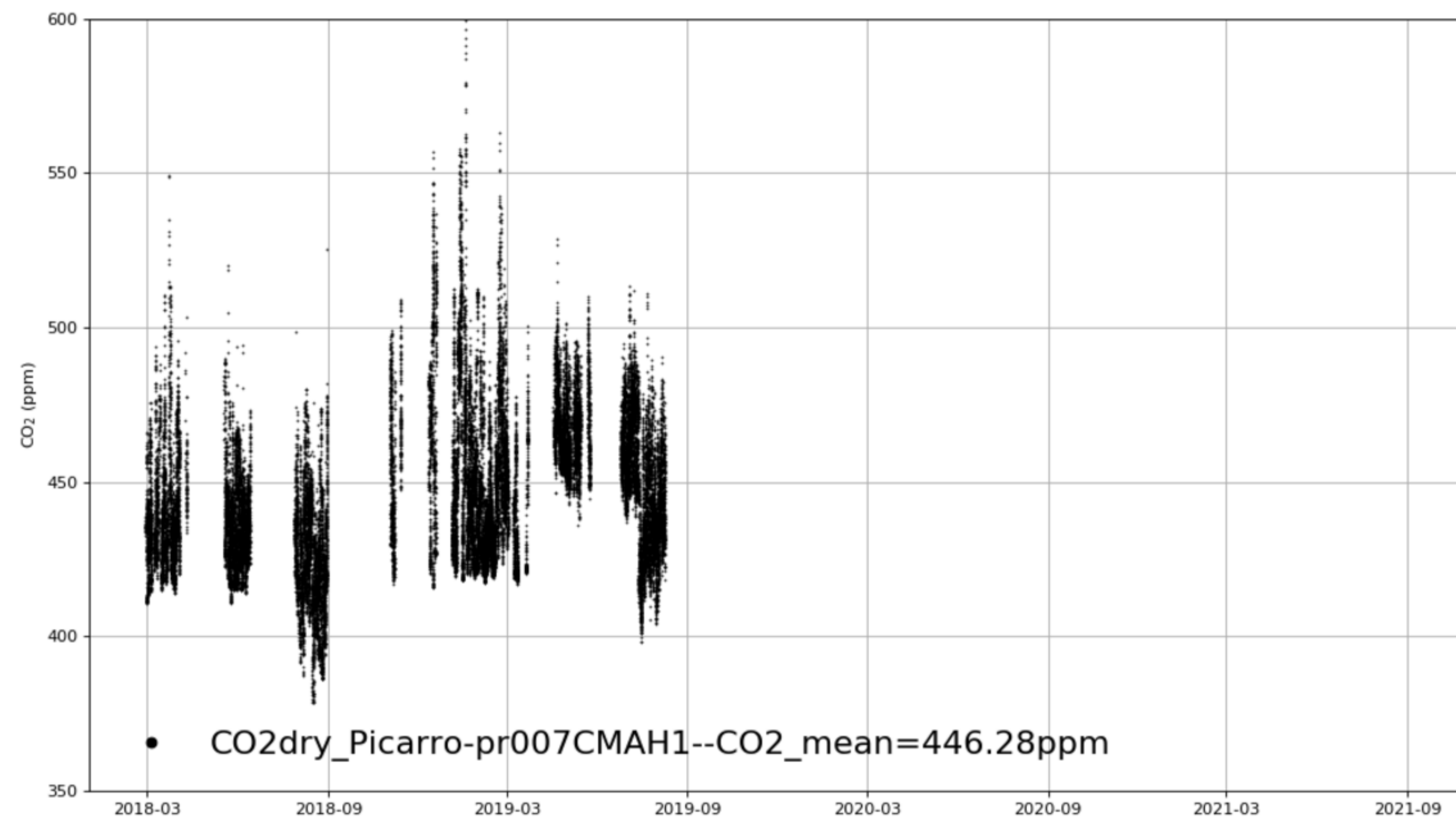
TJ_TianjinTower_CMAH1 tenmin/L2.0 for 3-years
