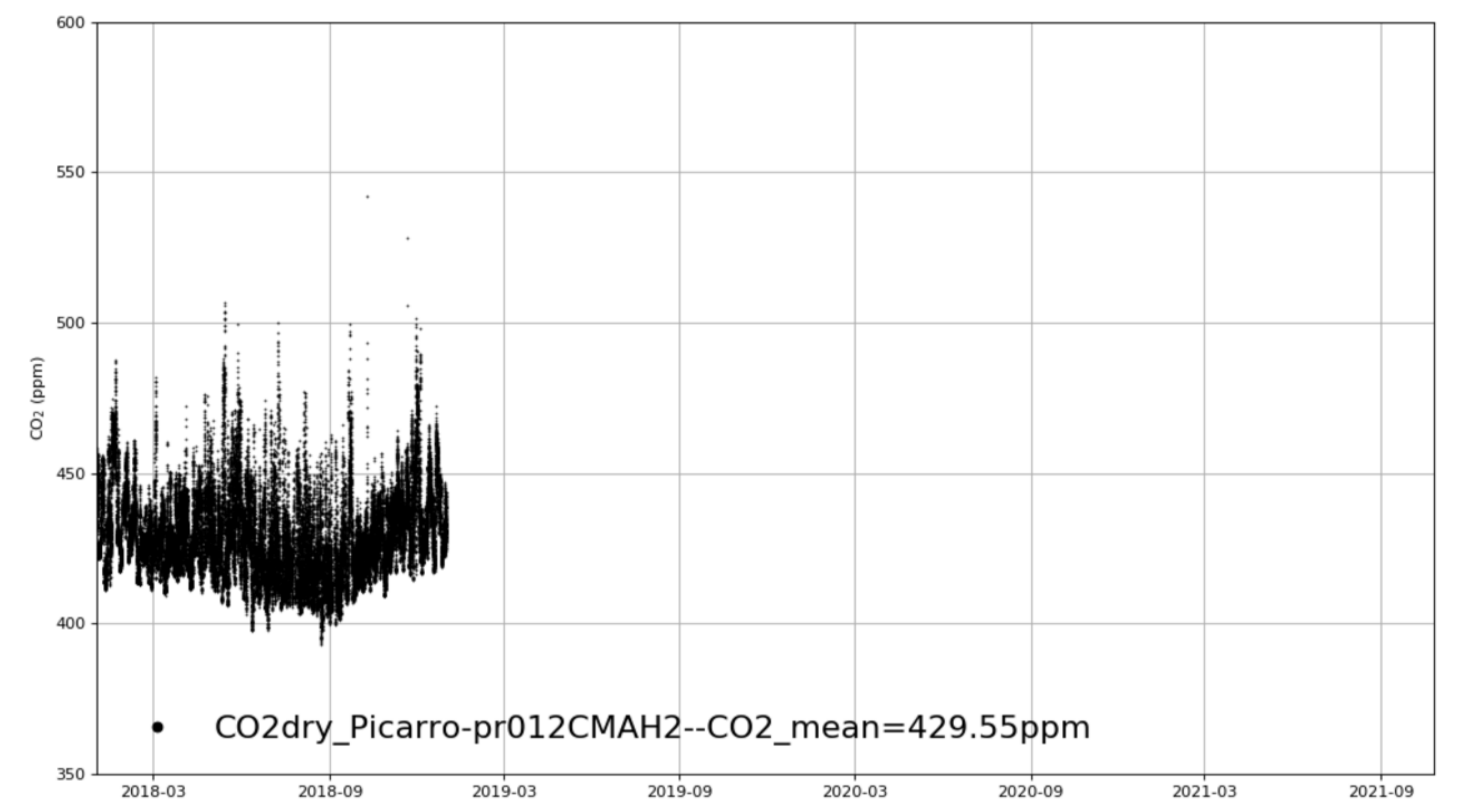
ZJ_LinAn_CMAH2 tenmin/L2.0 for 3-years
