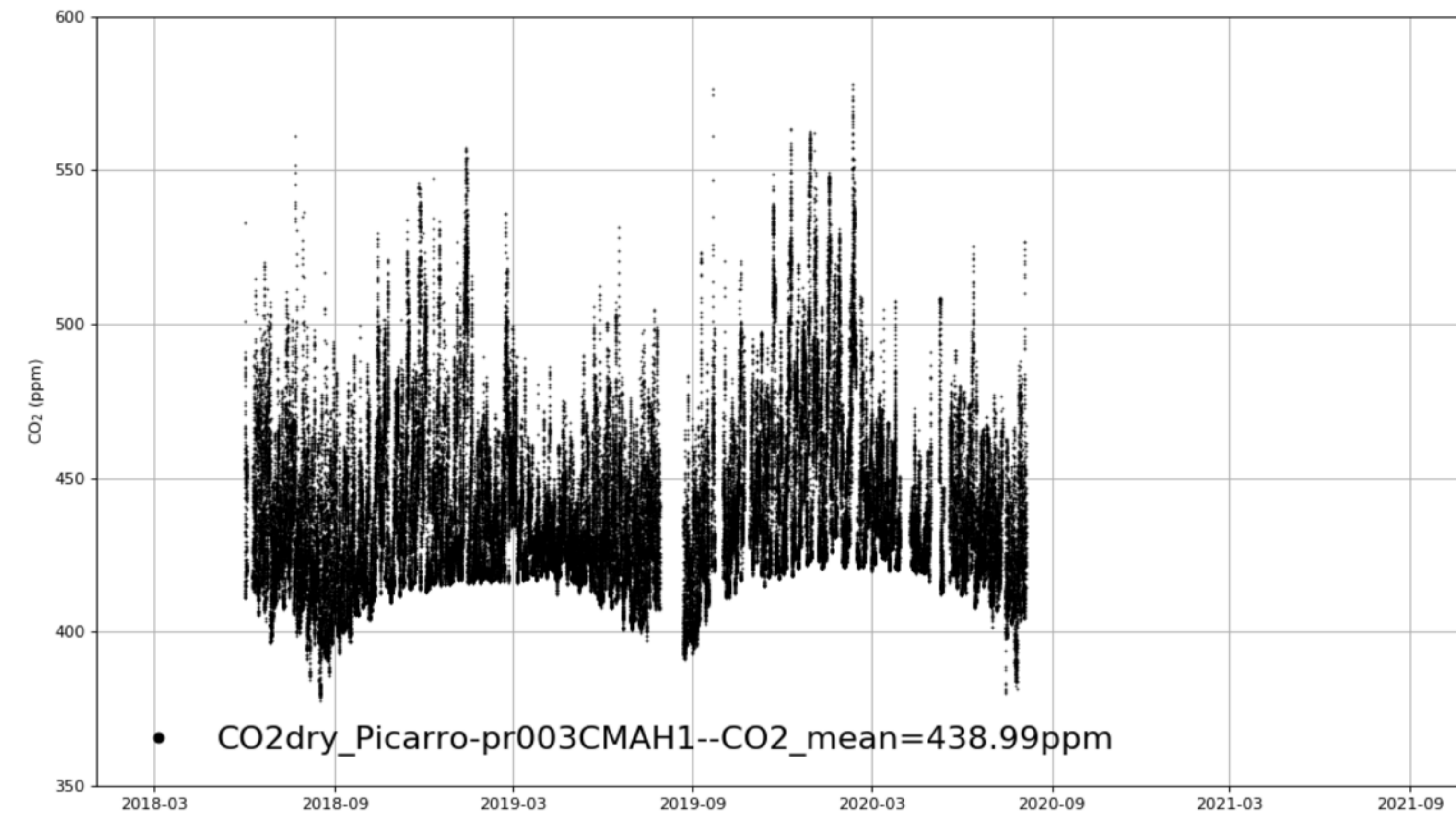
HE_Xianghe_CMAH1 tenmin/L2.0 for 3-years
