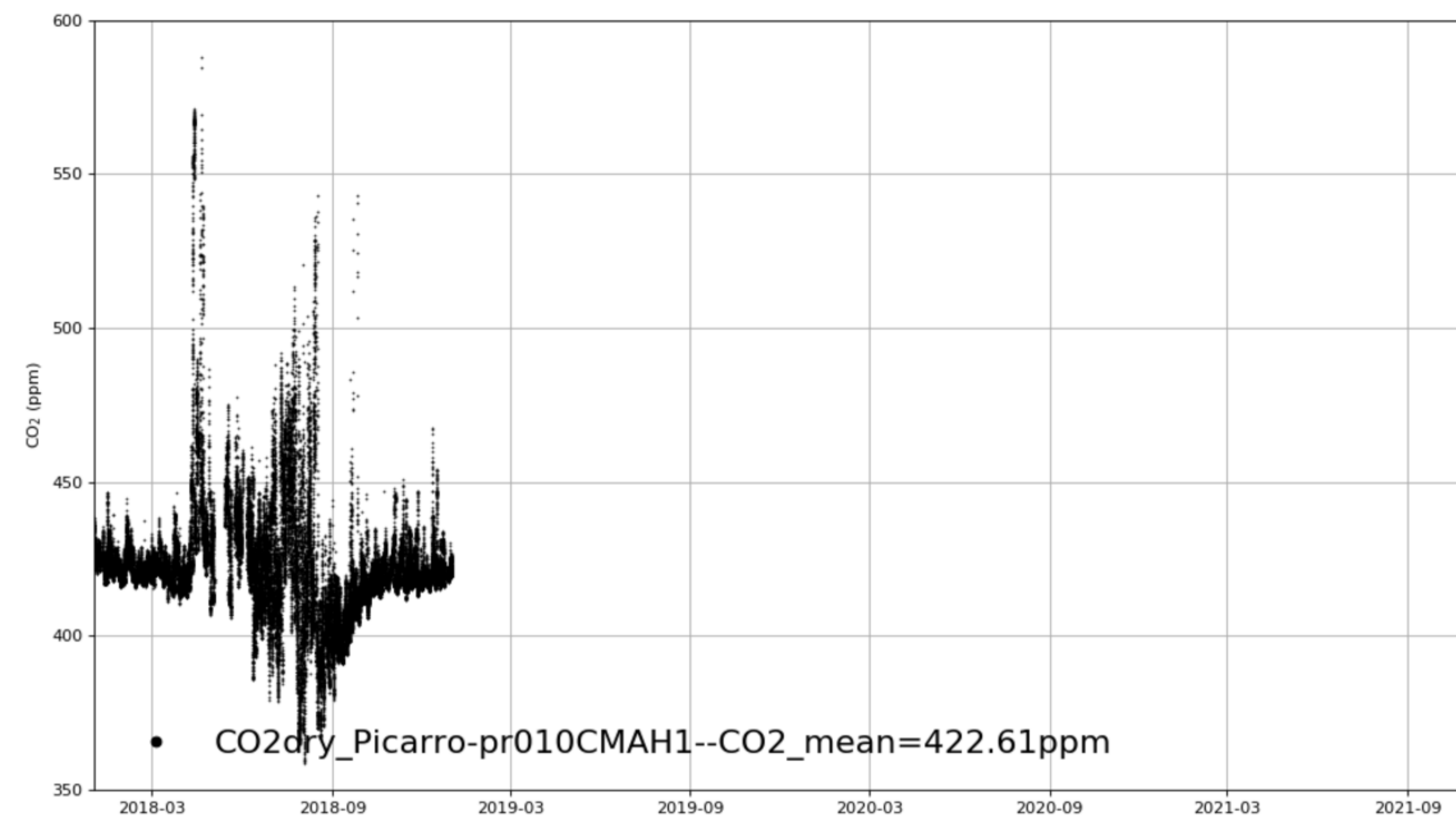
HL_Longfengshan_CMAH1 tenmin/L2.0 for 3-years
