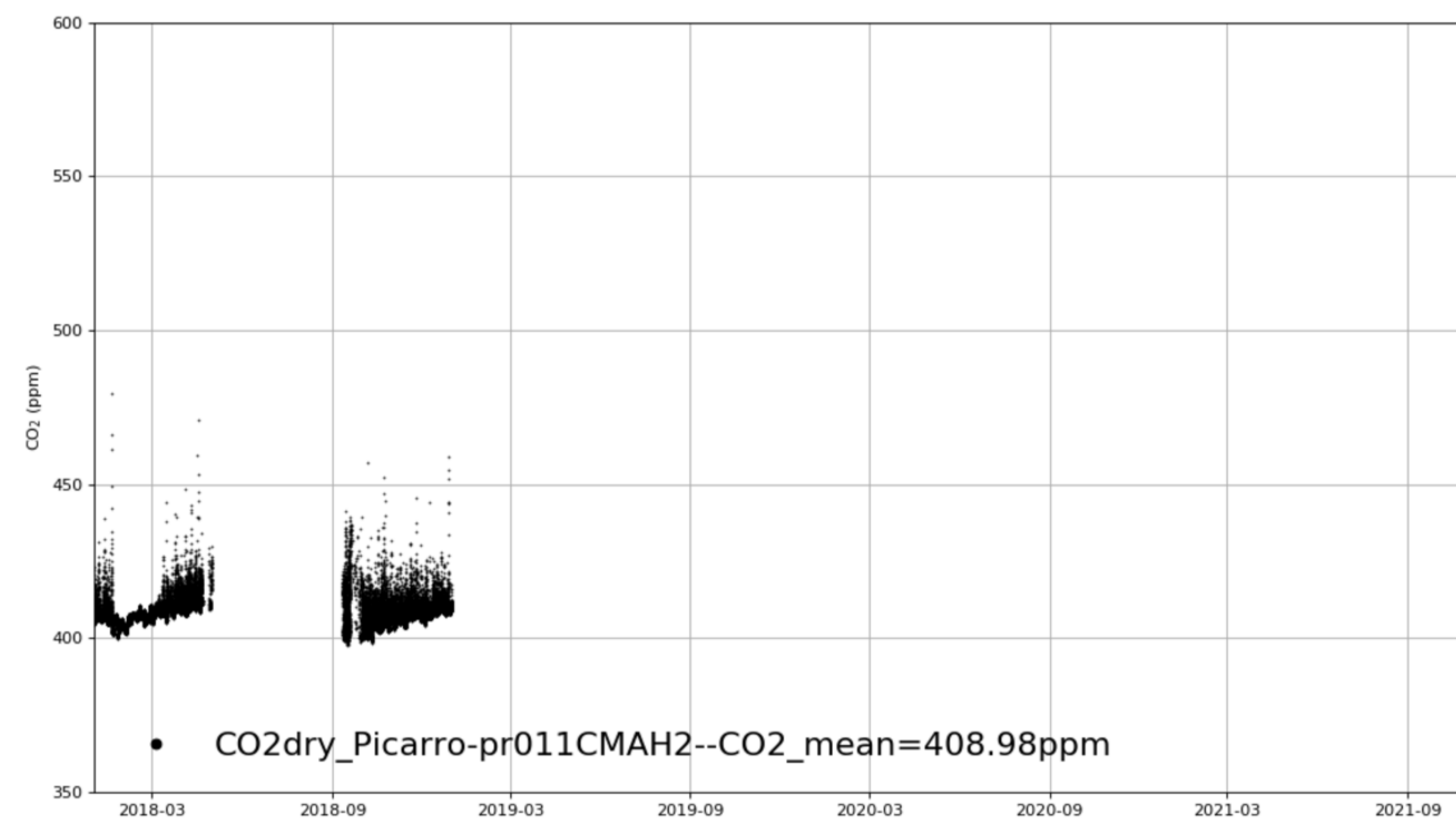
YN_Xianggelila_CMAH2 tenmin/L2.0 for 3-years
