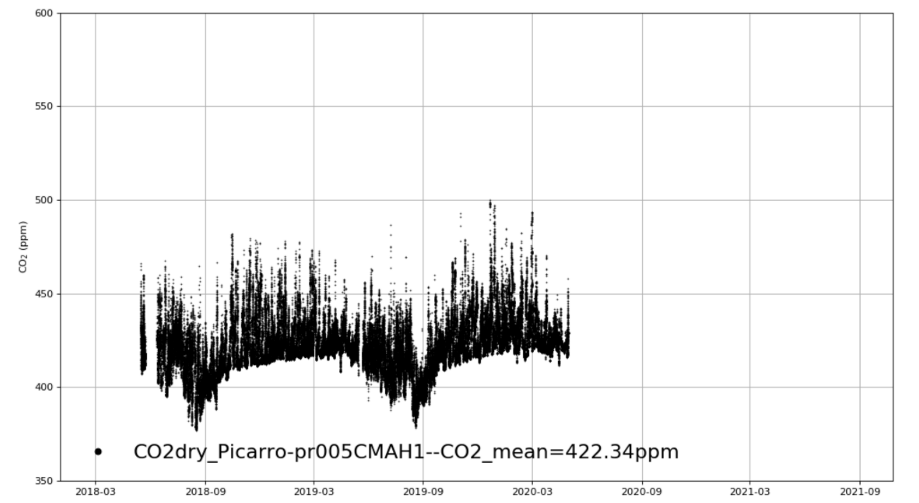
HE_Xinglong_CMAH1 tenmin/L2.0 for 3-years
