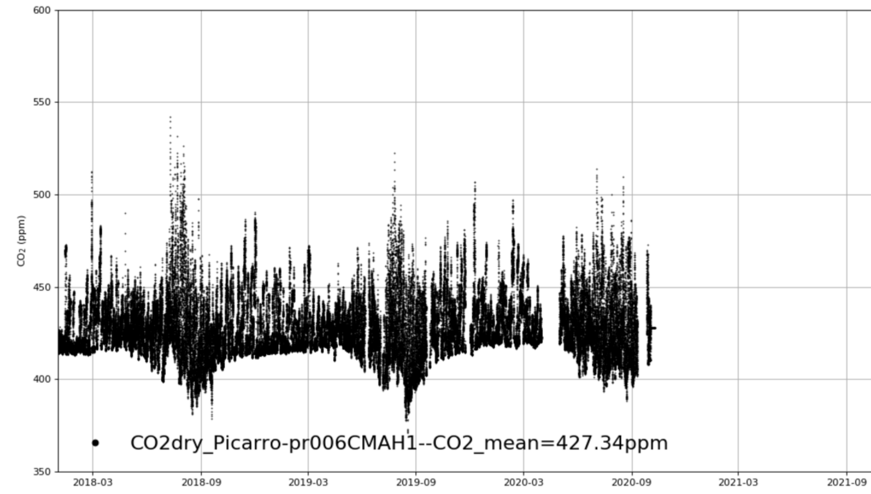
BJ_Shangdianzi_CMAH1 tenmin/L2.0 for 3-years
