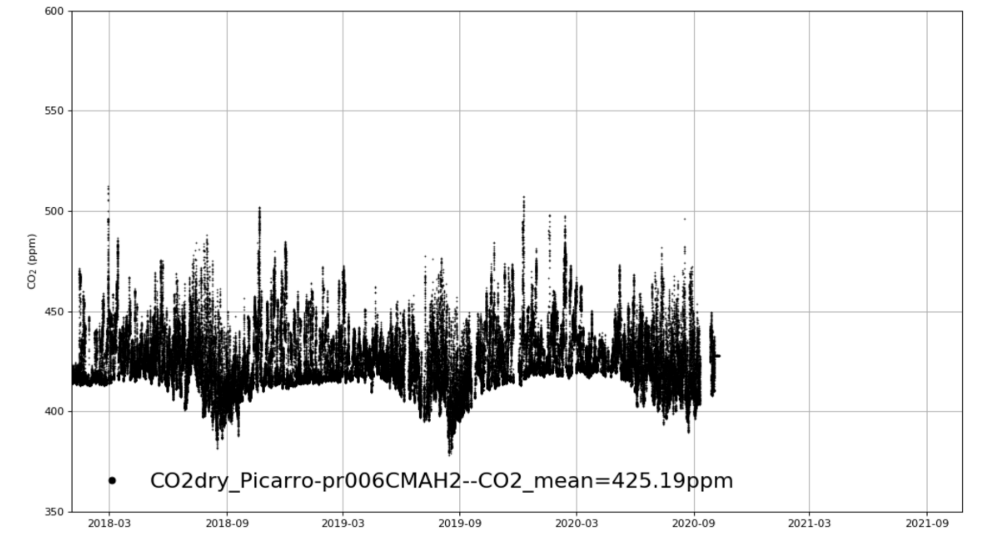
BJ_Shangdianzi_CMAH2 tenmin/L2.0 for 3-years
