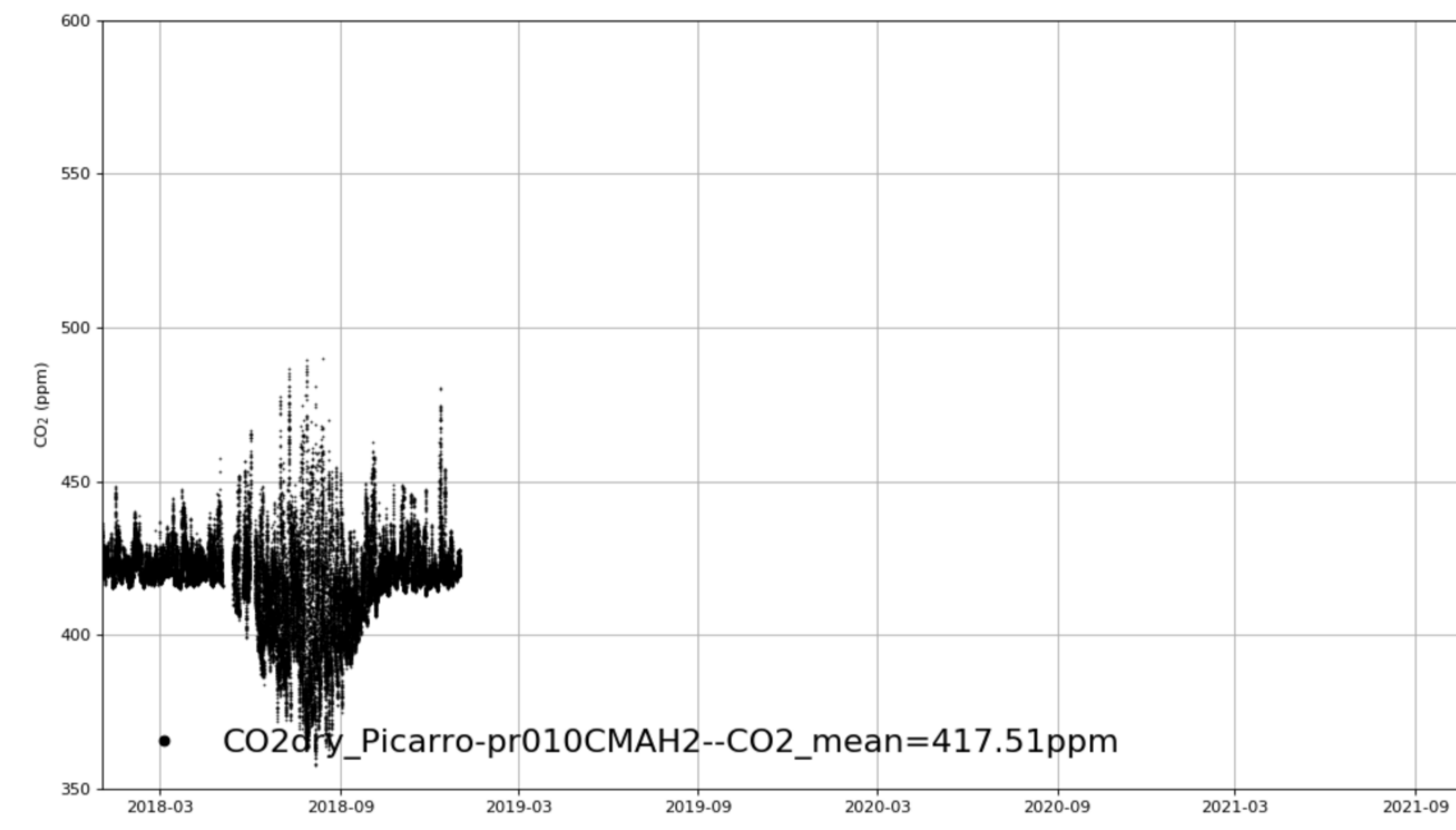
HL_Longfengshan_CMAH2 tenmin/L2.0 for 3-years
