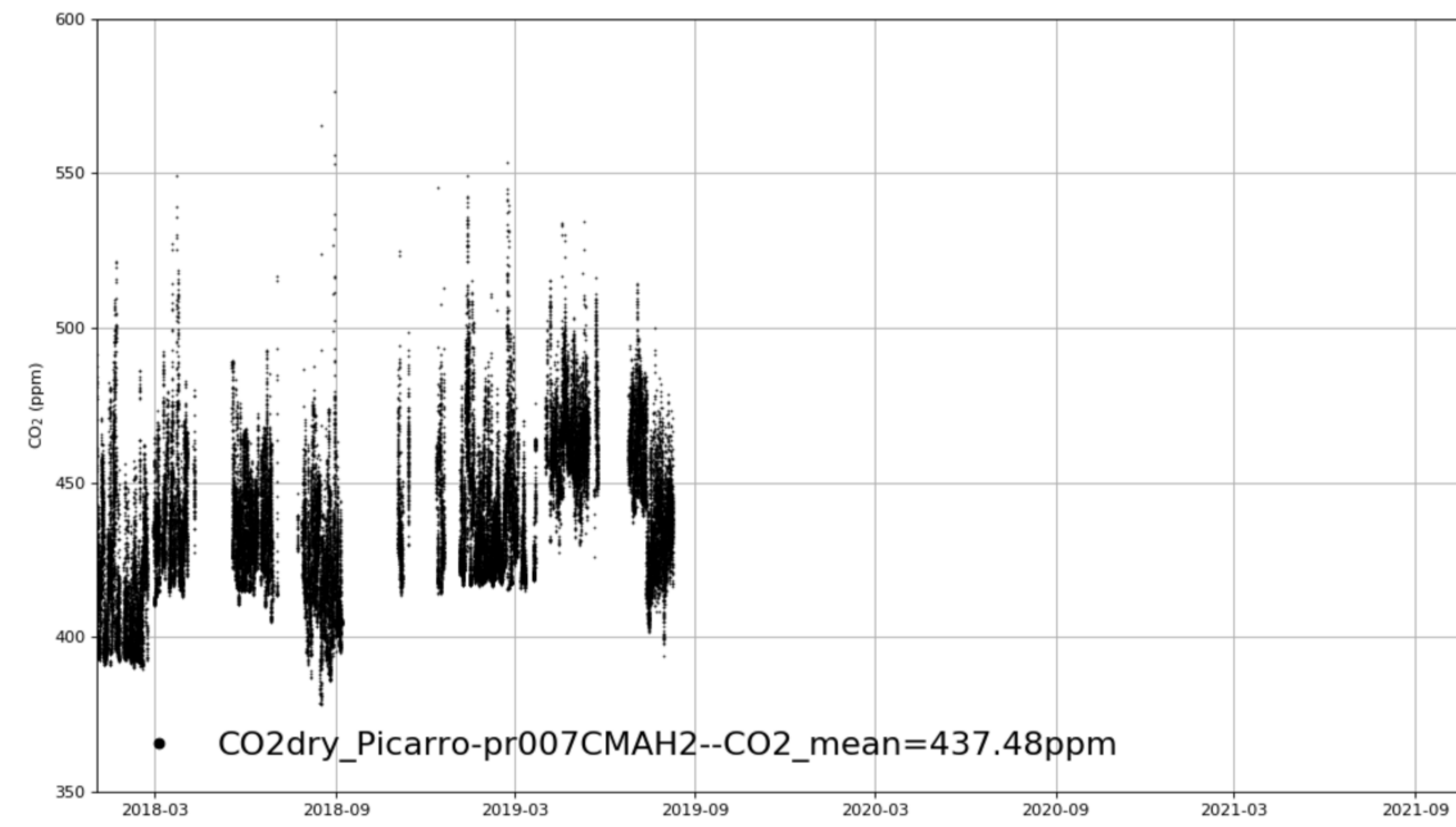
TJ_TianjinTower_CMAH2 tenmin/L2.0 for 3-years
