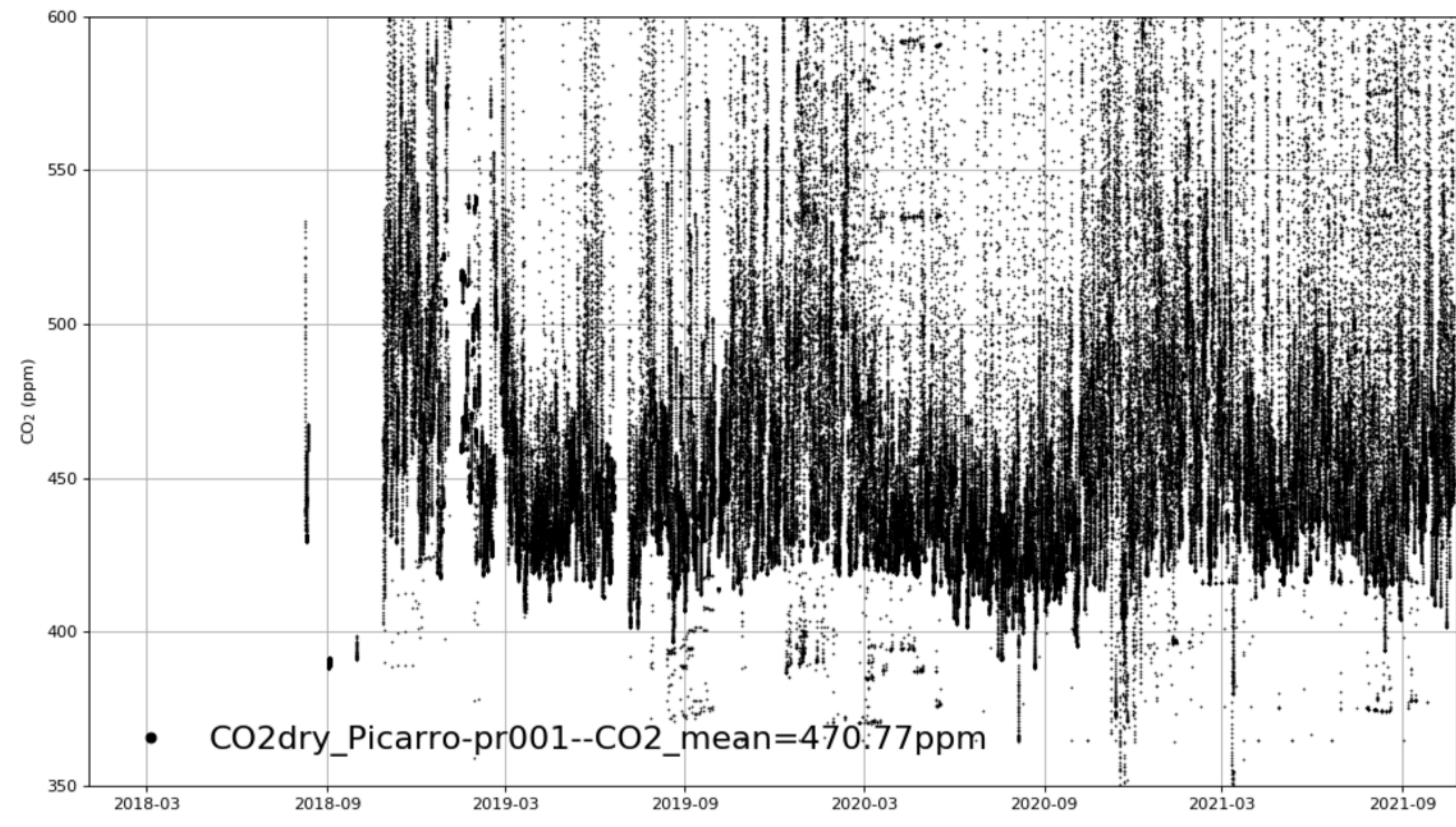
BJ_IAPLab617 tenmin/L2.0 for 3-years
