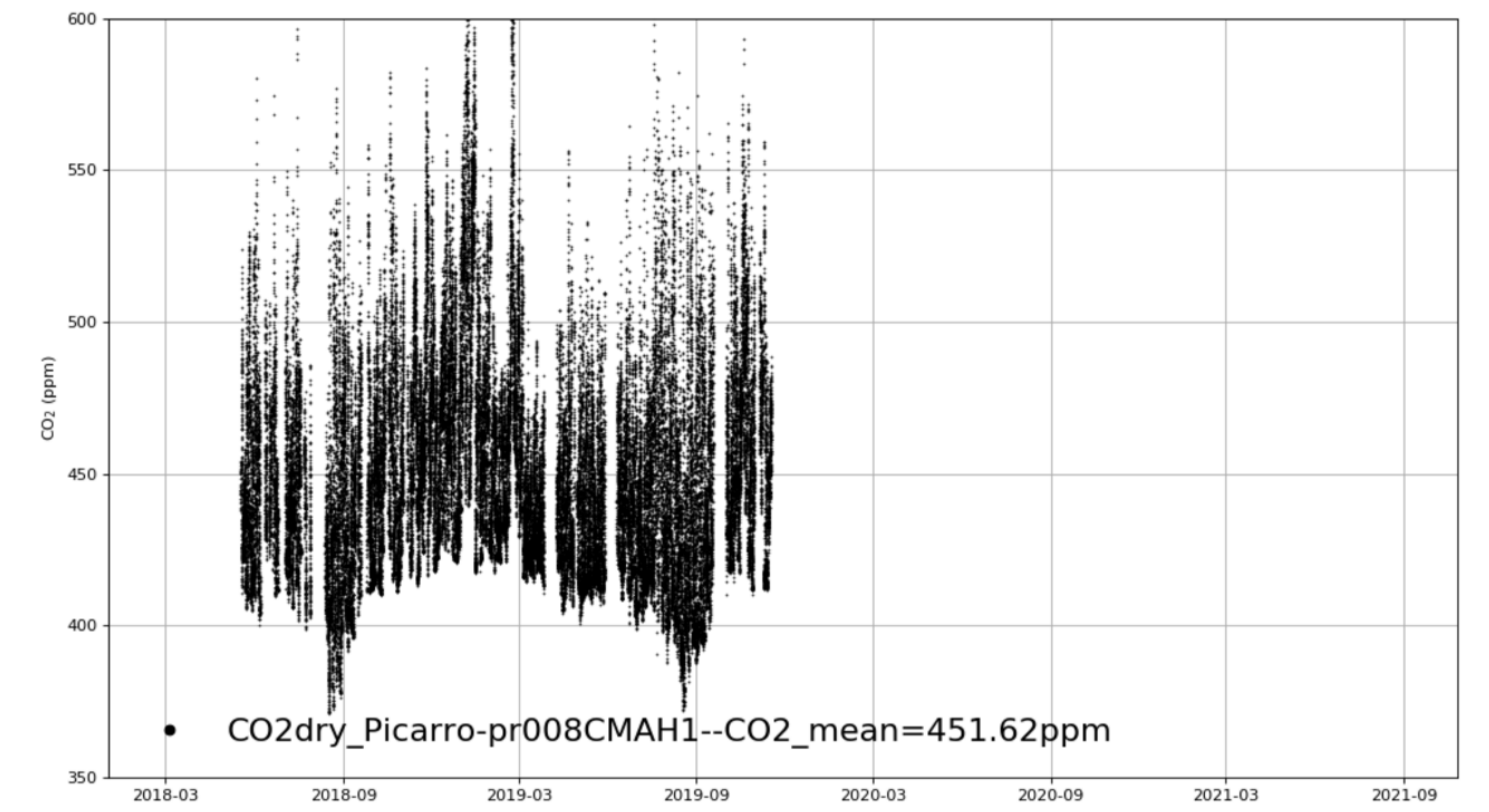
HE_Luancheng_CMAH1 tenmin/L2.0 for 3-years
