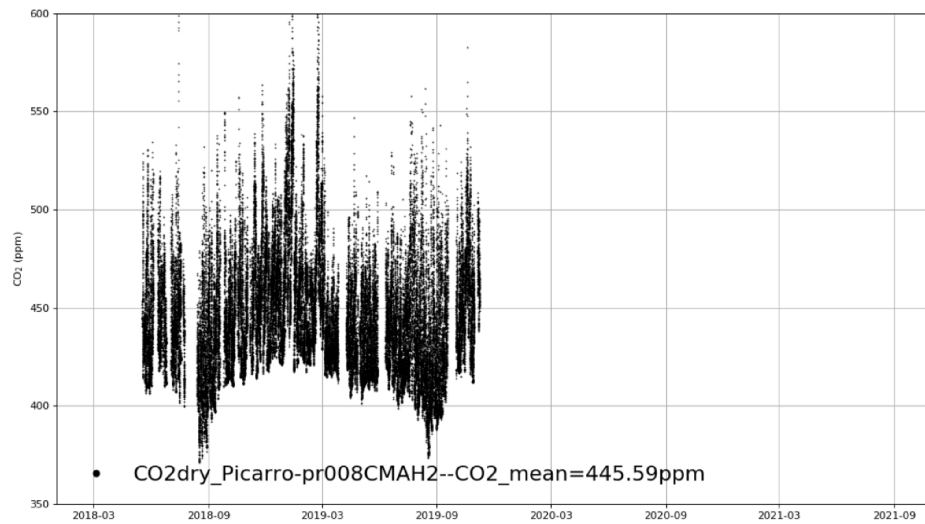
HE_Luancheng_CMAH2 tenmin/L2.0 for 3-years
