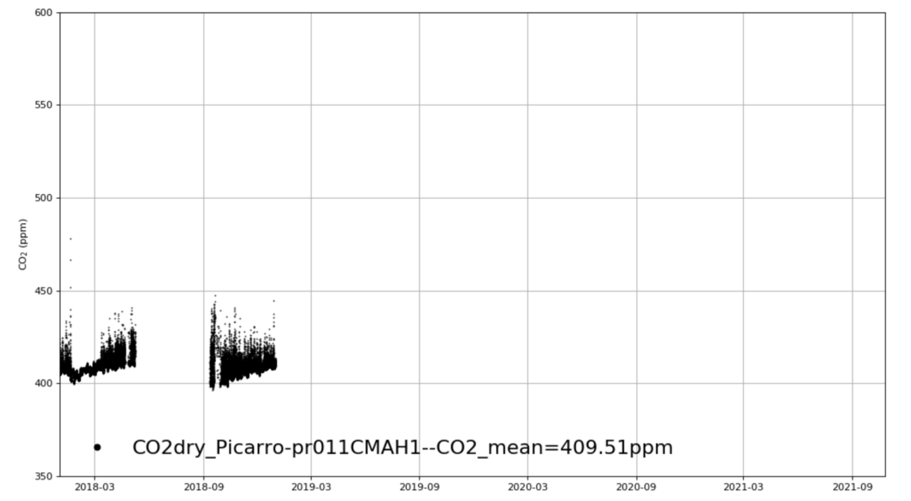
YN_Xianggelila_CMAH1 tenmin/L2.0 for 3-years
