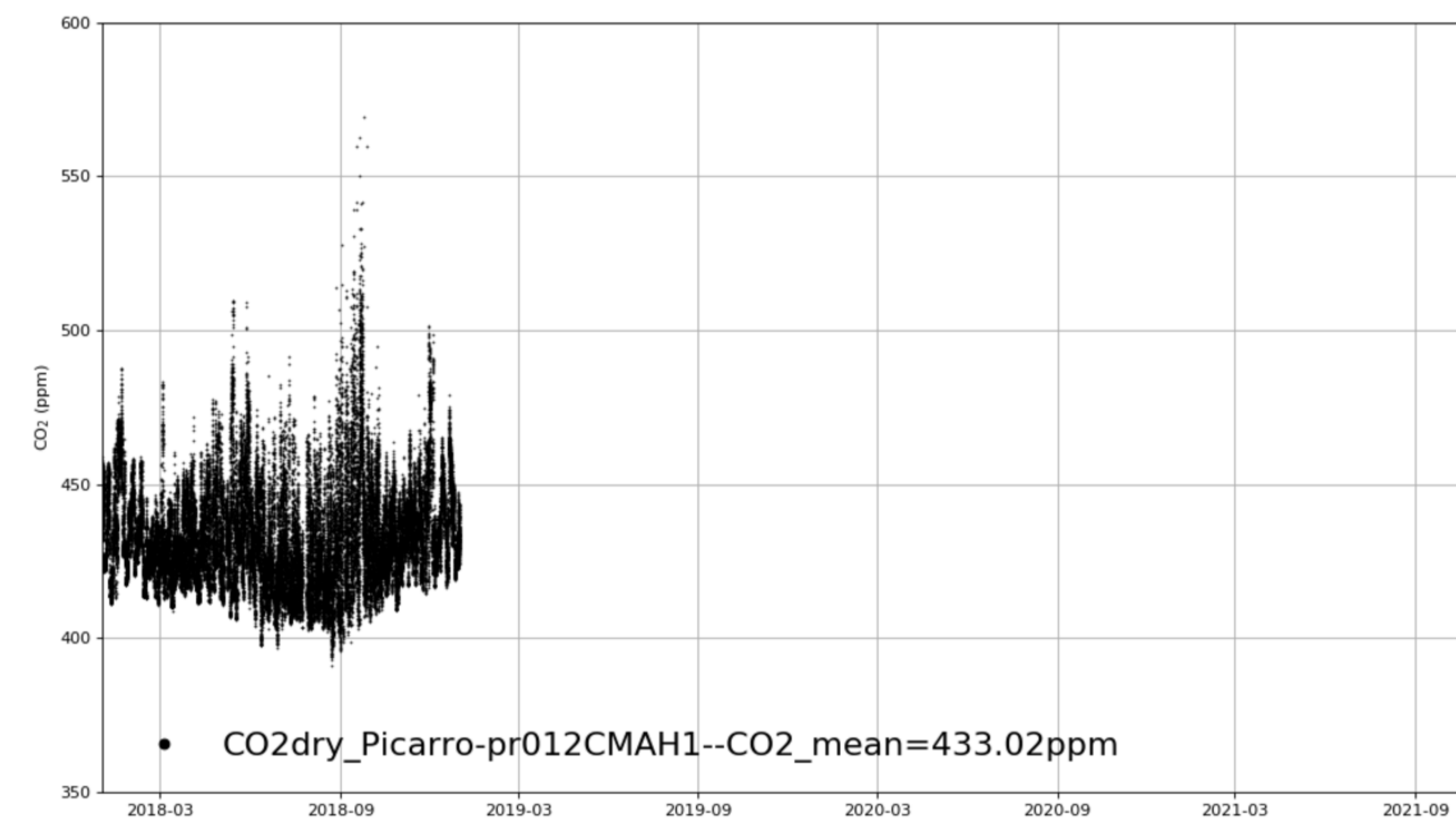
ZJ_LinAn_CMAH1 tenmin/L2.0 for 3-years
