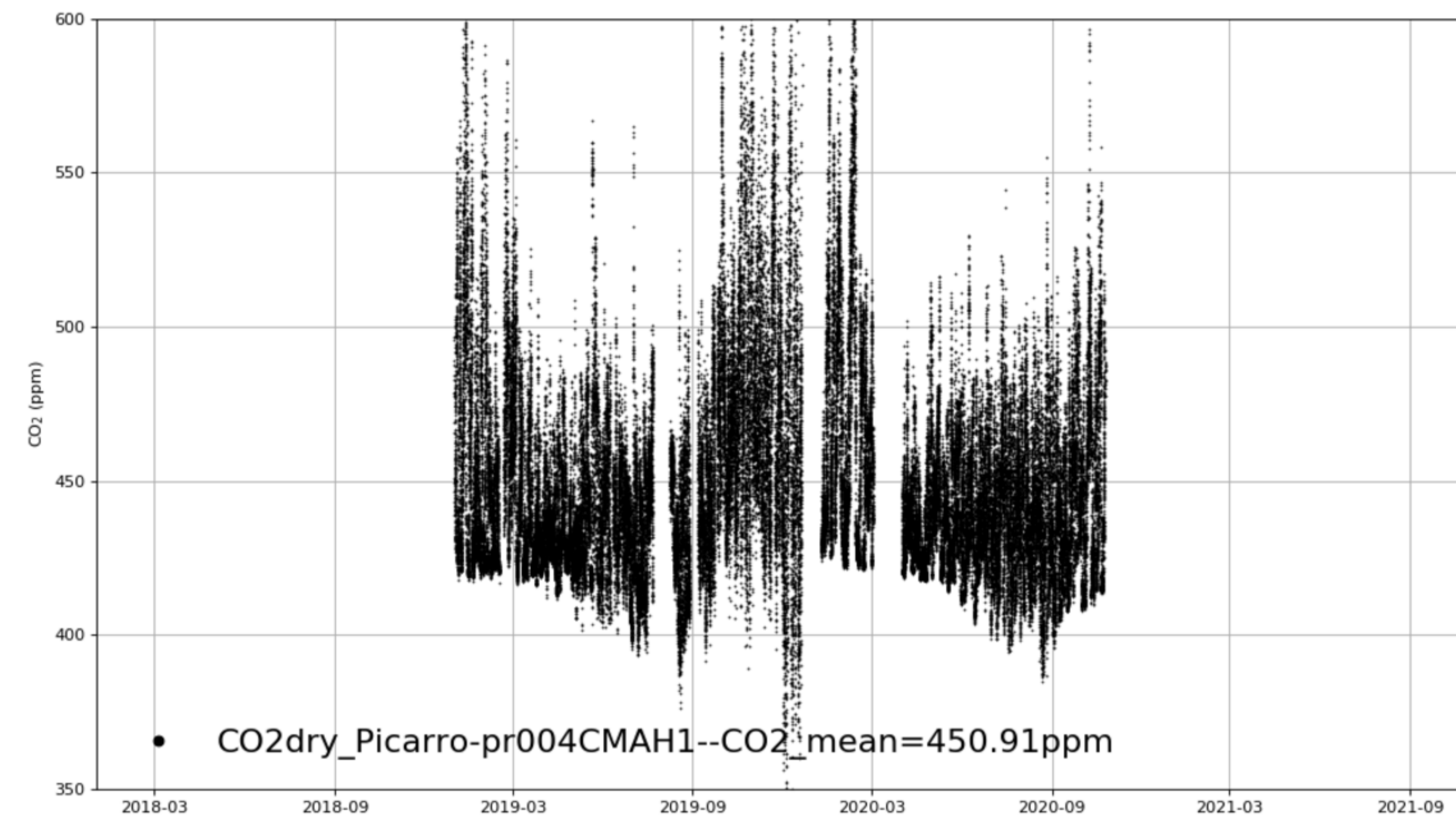
BJ_IAPTower_CMAH1 tenmin/L2.0 for 3-years
