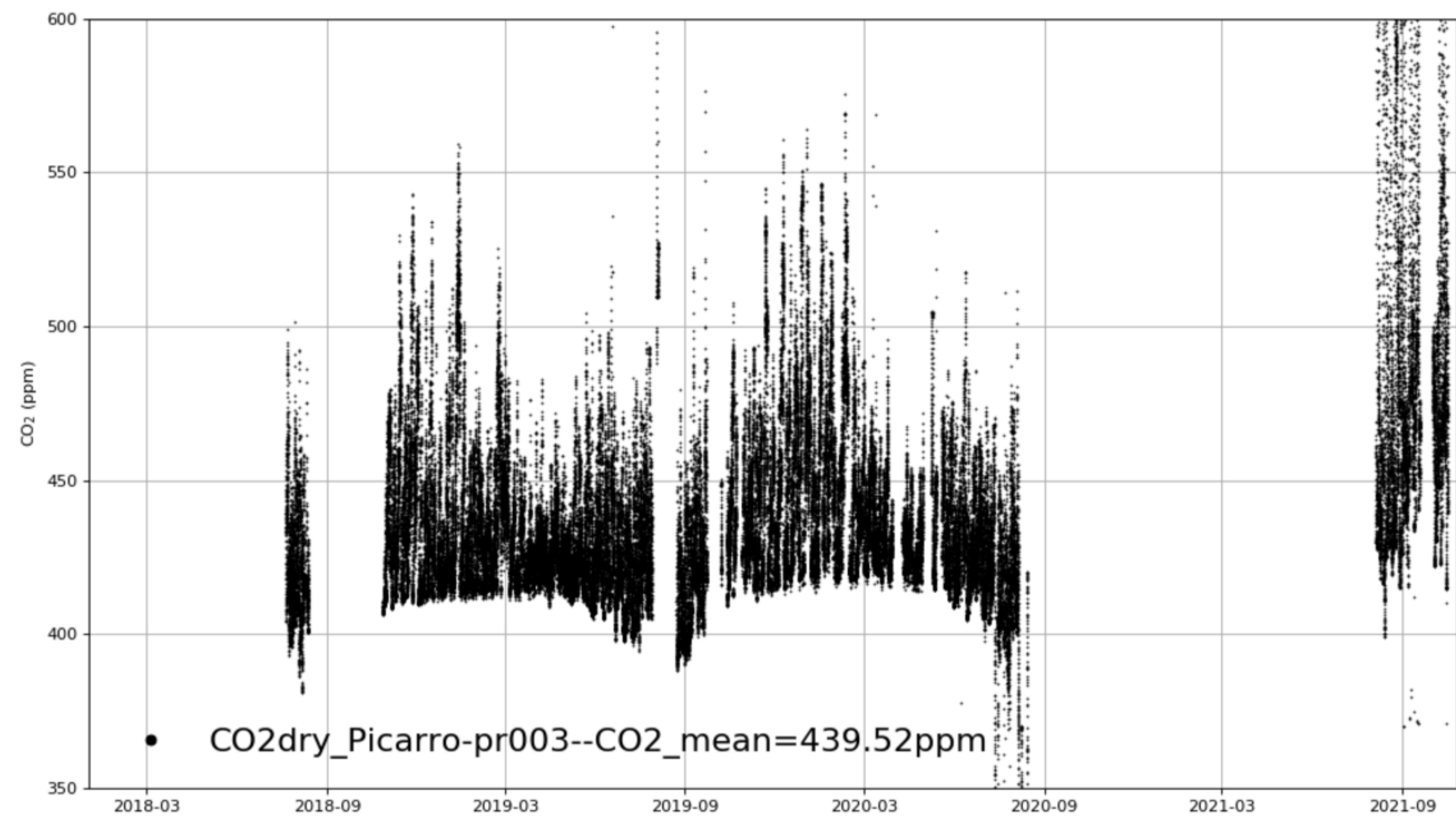
HE_Xianghe_BB tenmin/L2.0 for 3-years
