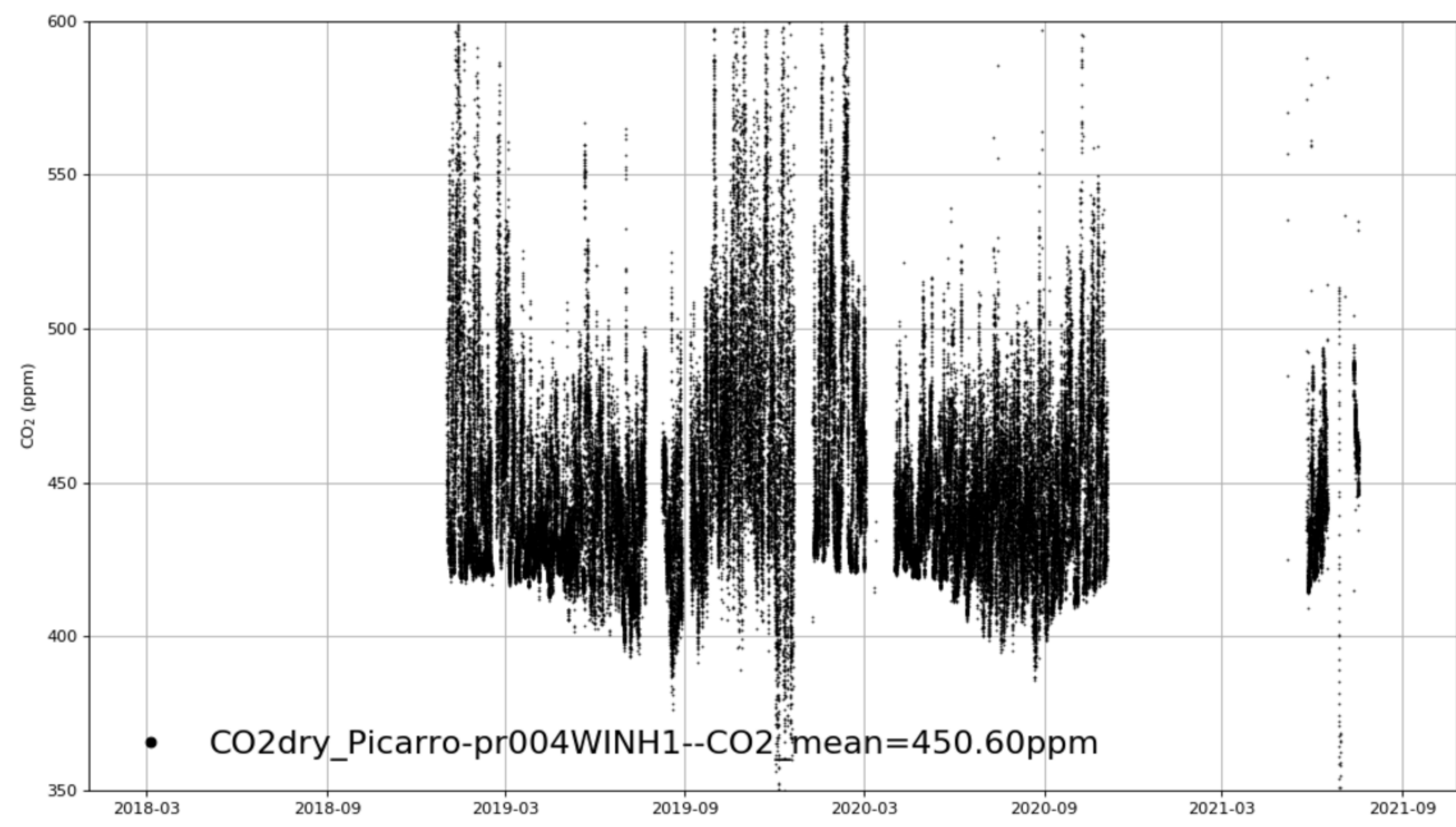
BJ_IAPTower_WINH1 tenmin/L2.0 for 3-years
