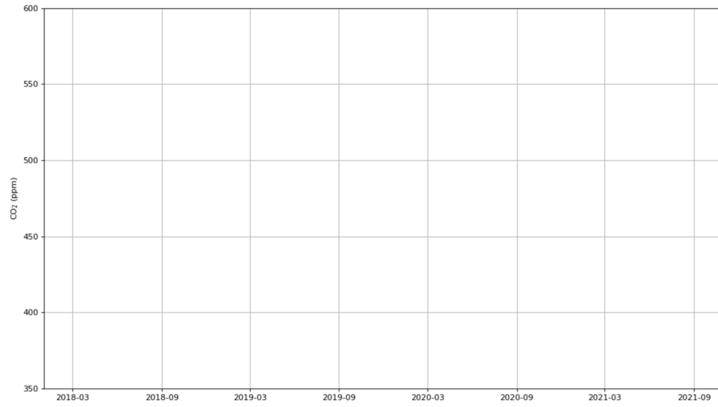
HE_Xinglong_CMAH2 tenmin/L2.0 for 3-years
