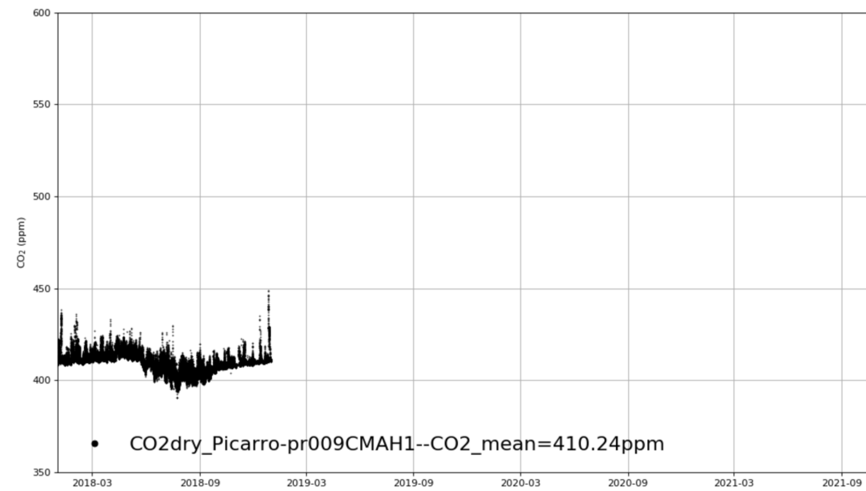
QH_Waliguan_CMAH1 tenmin/L2.0 for 3-years
