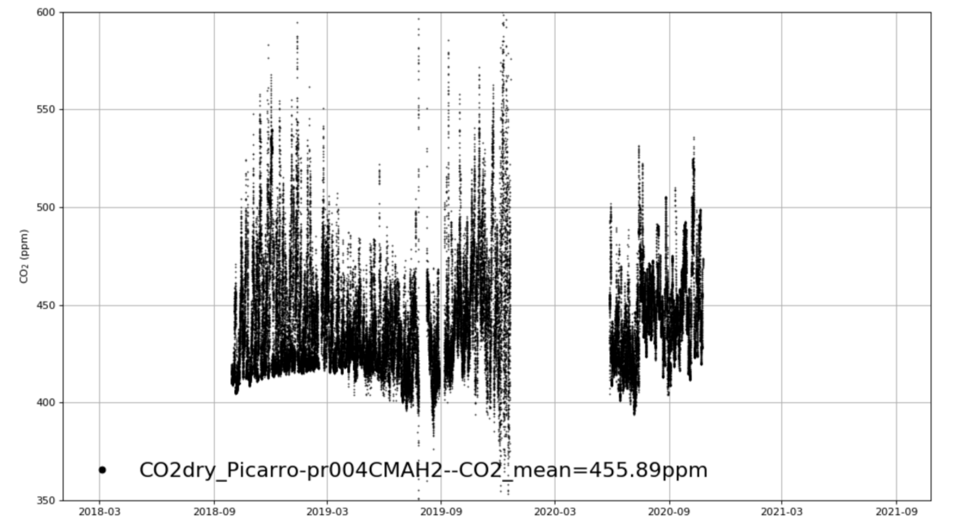
BJ_IAPTower_CMAH2 tenmin/L2.0 for 3-years
