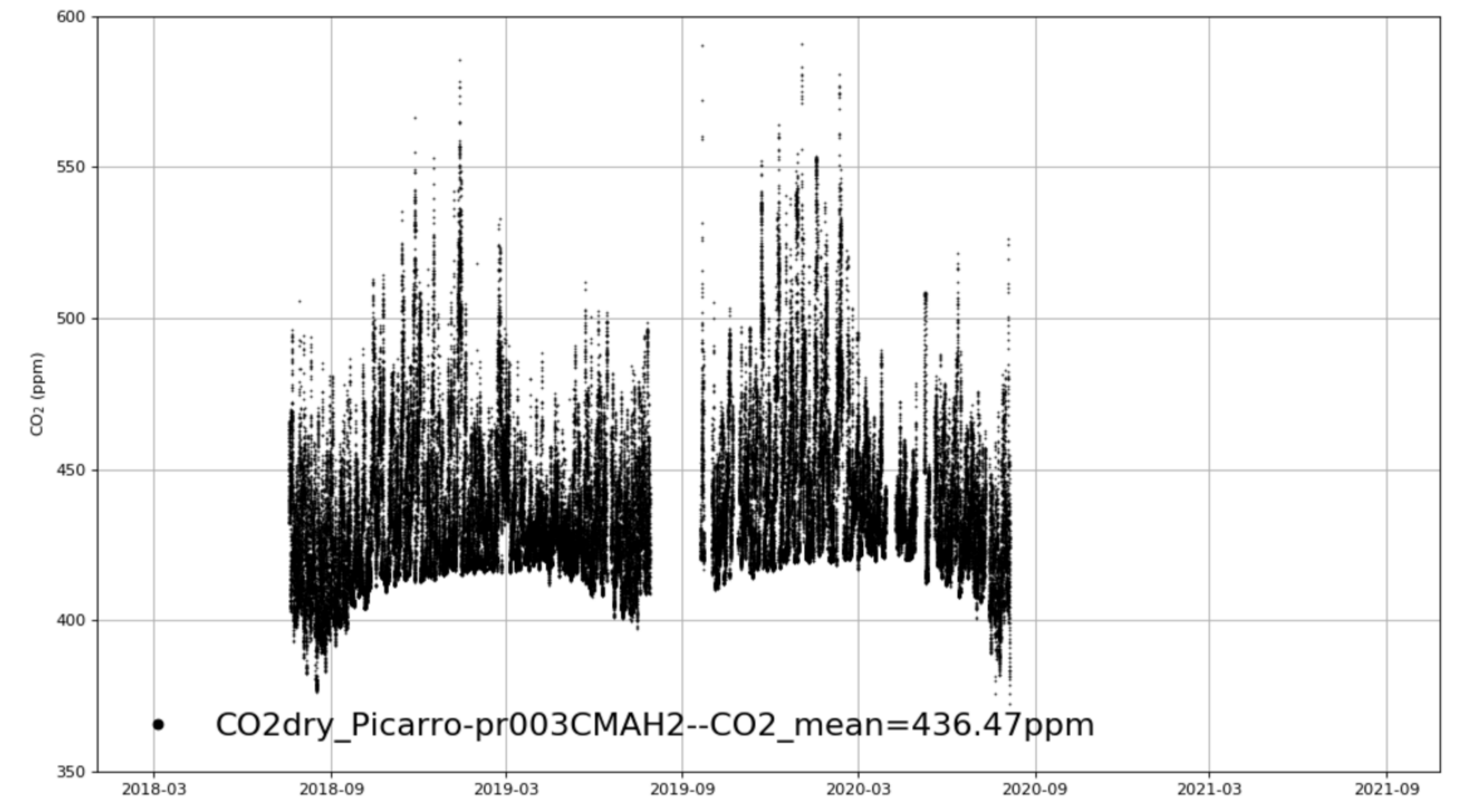
HE_Xianghe_CMAH2 tenmin/L2.0 for 3-years
