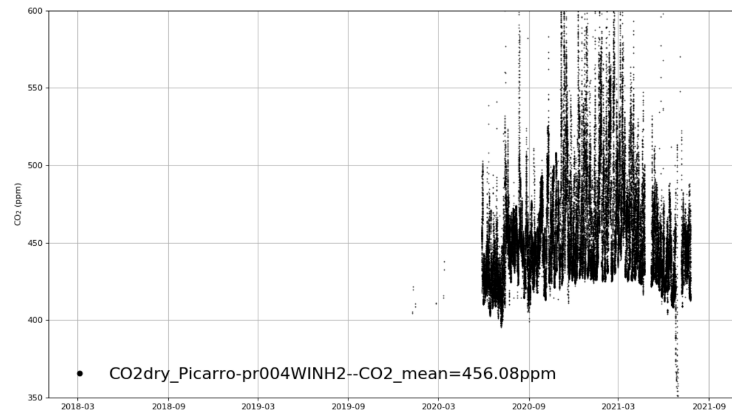
BJ_IAPTower_WINH2 tenmin/L2.0 for 3-years
