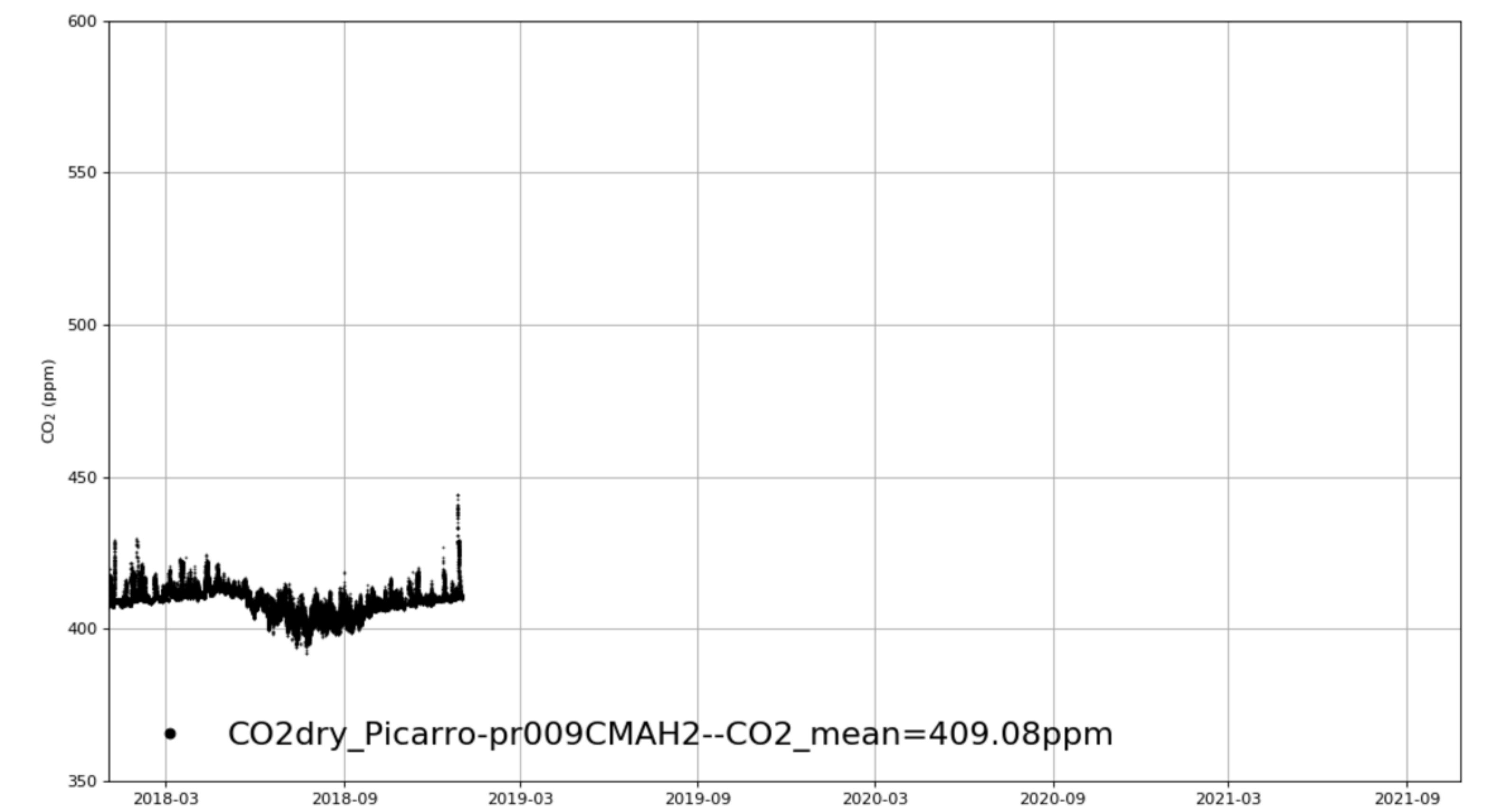
QH_Waliguan_CMAH2 tenmin/L2.0 for 3-years
